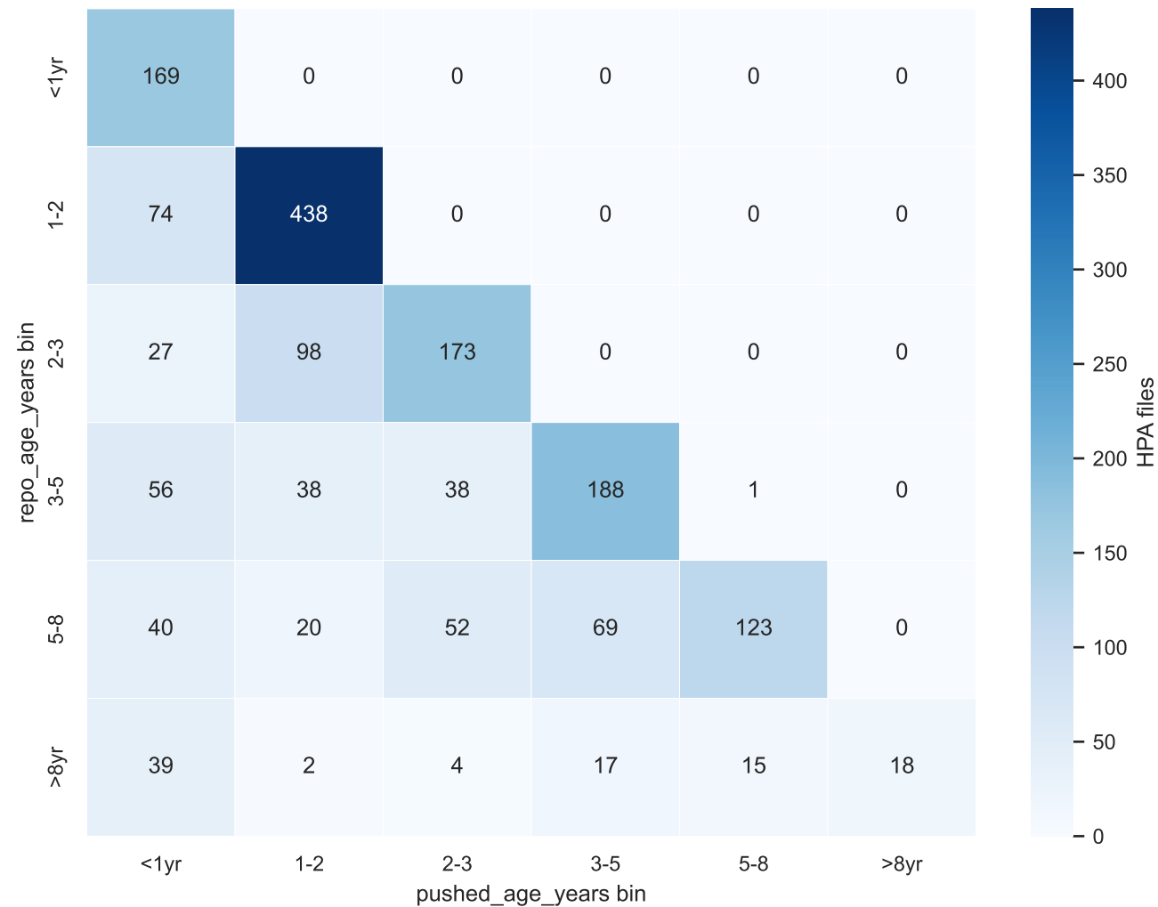
repo_age vs. pushed_age for v1 HPA files
