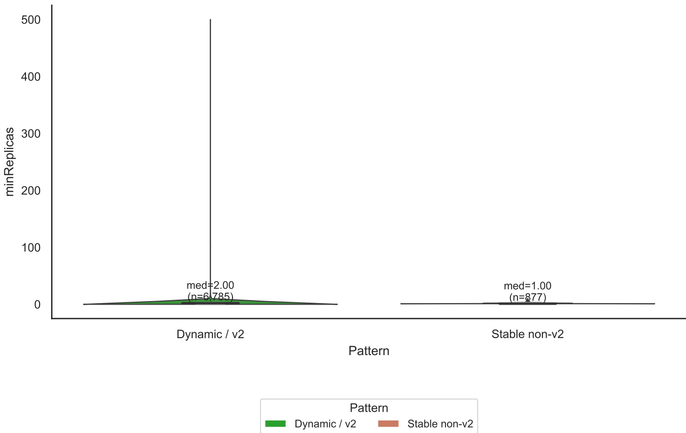
minReplicas in stable vs. dynamic HPAs
