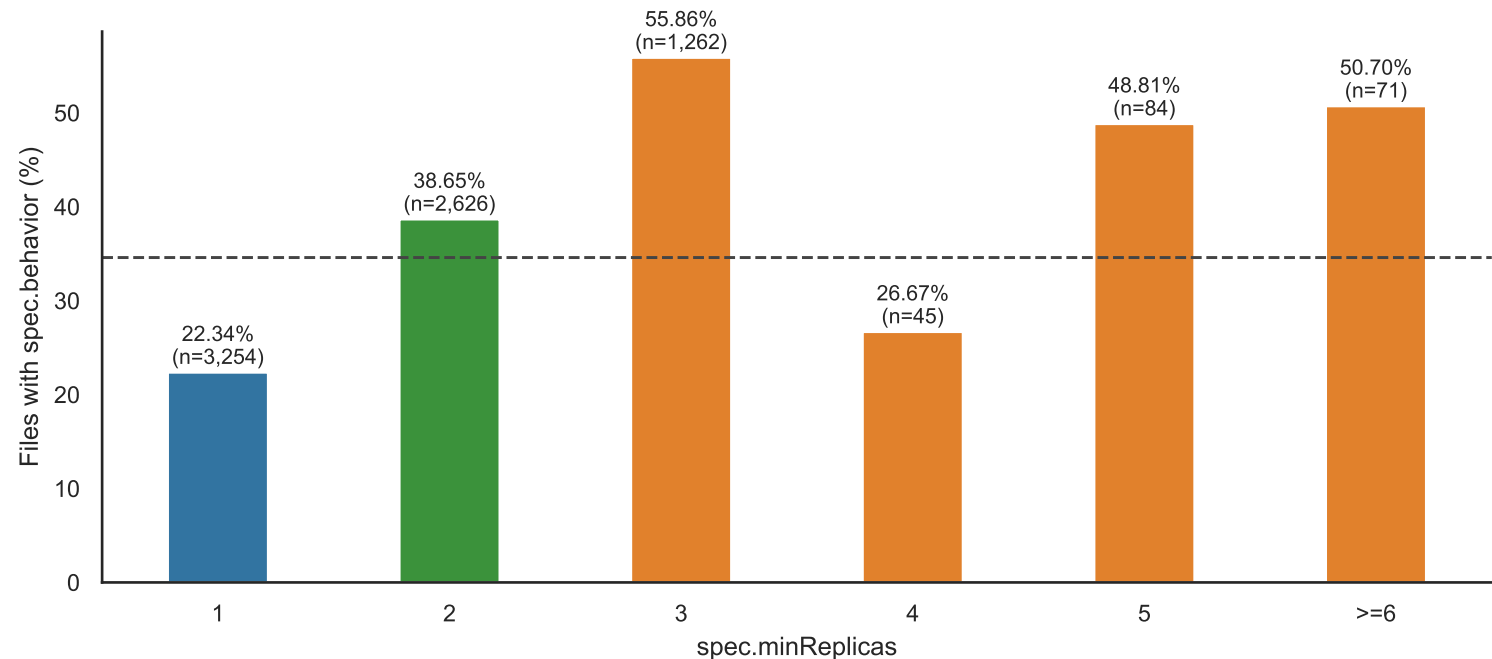
spec.behavior by minReplicas value
