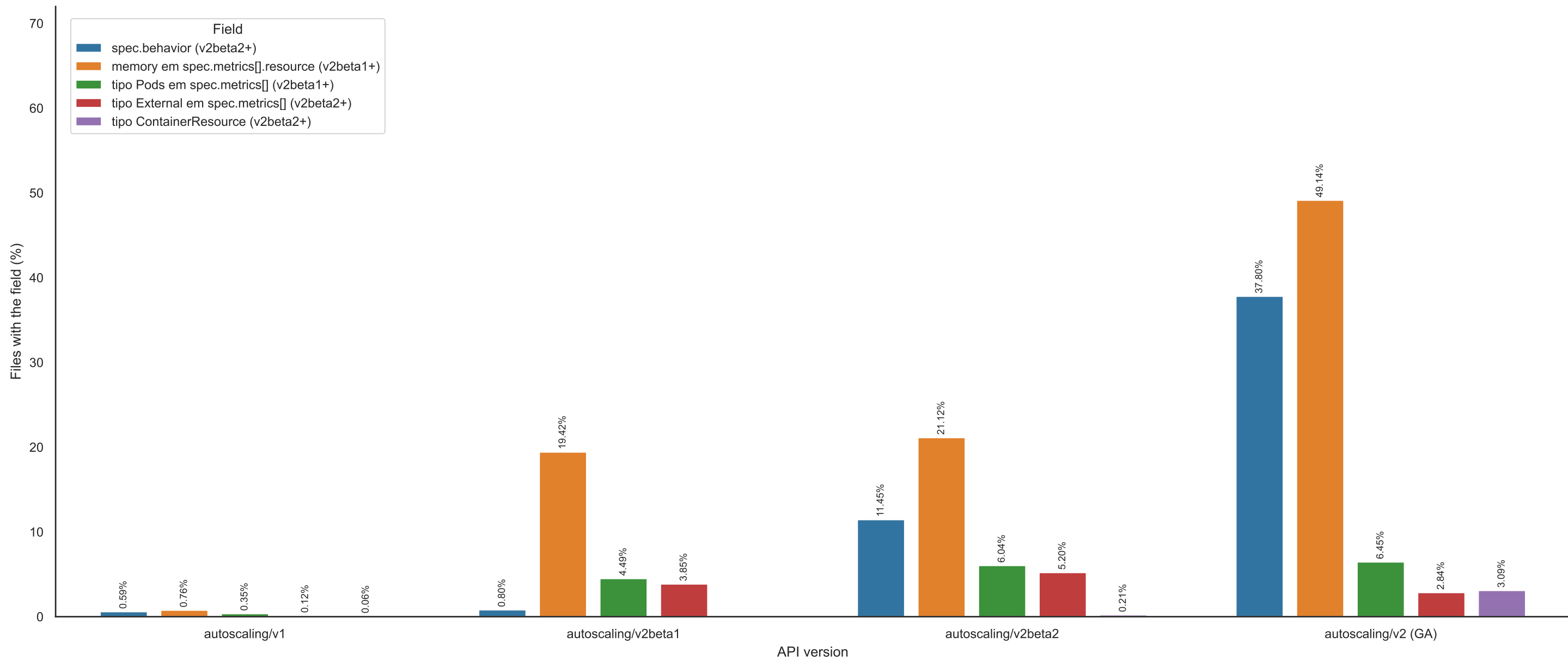
Adoption of optional fields by API version
