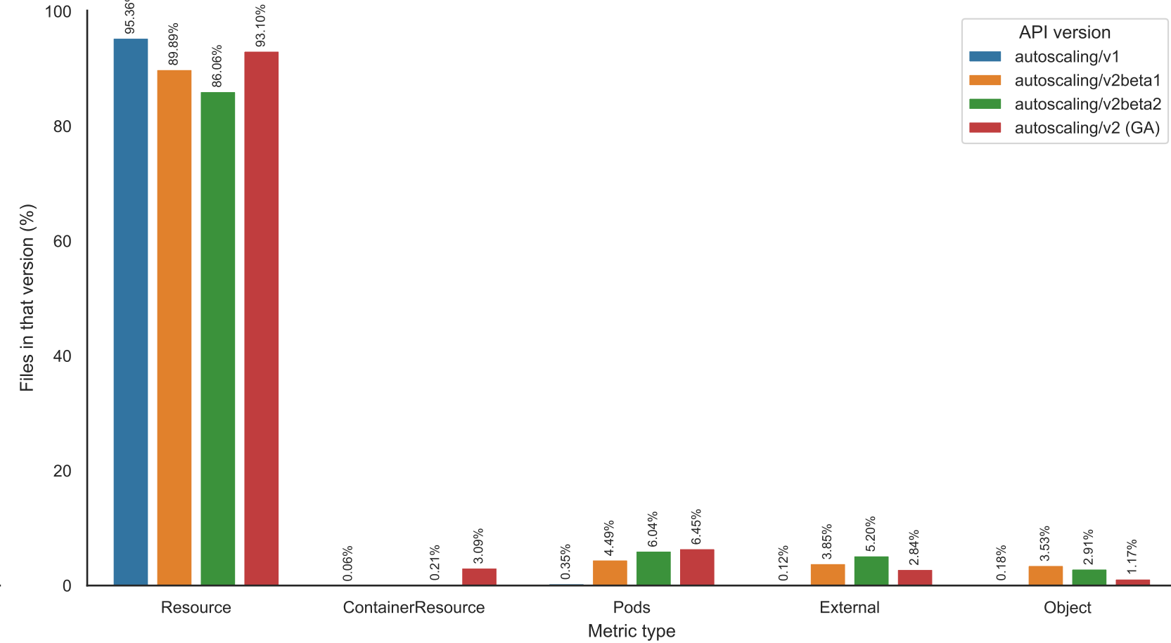
(B) Adoption by metric type and API version
