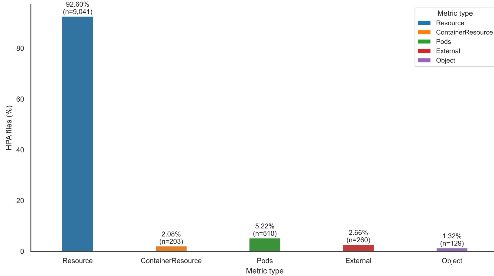
(A) Overall adoption of metric types
