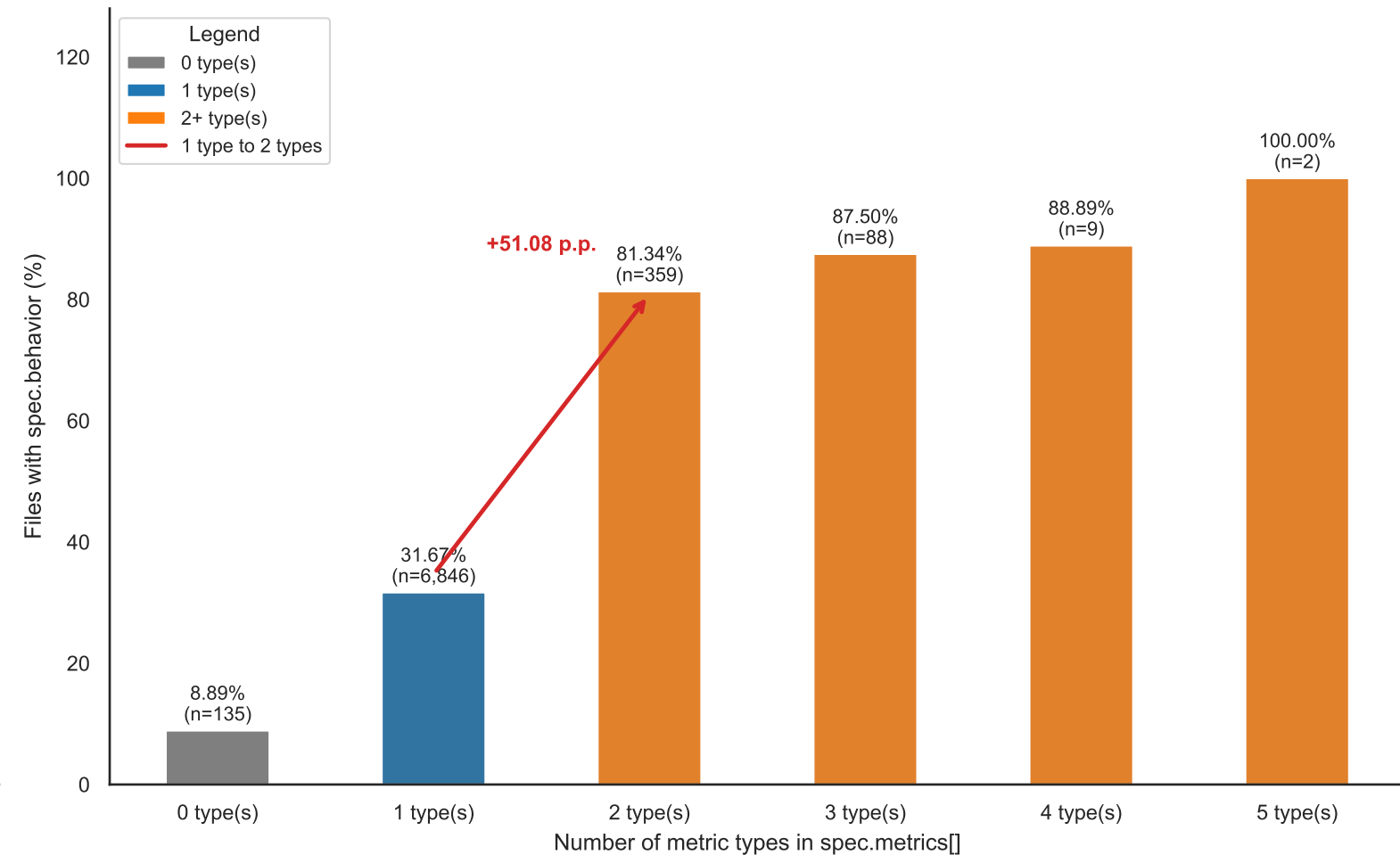
(B) spec.behavior adoption by metric type count
