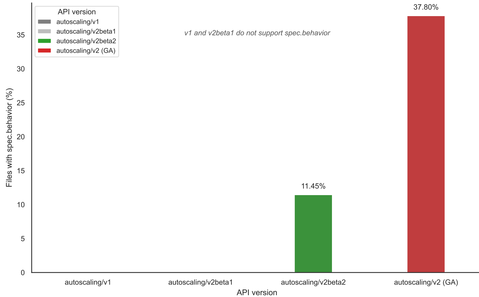
(A) spec.behavior adoption by API version
