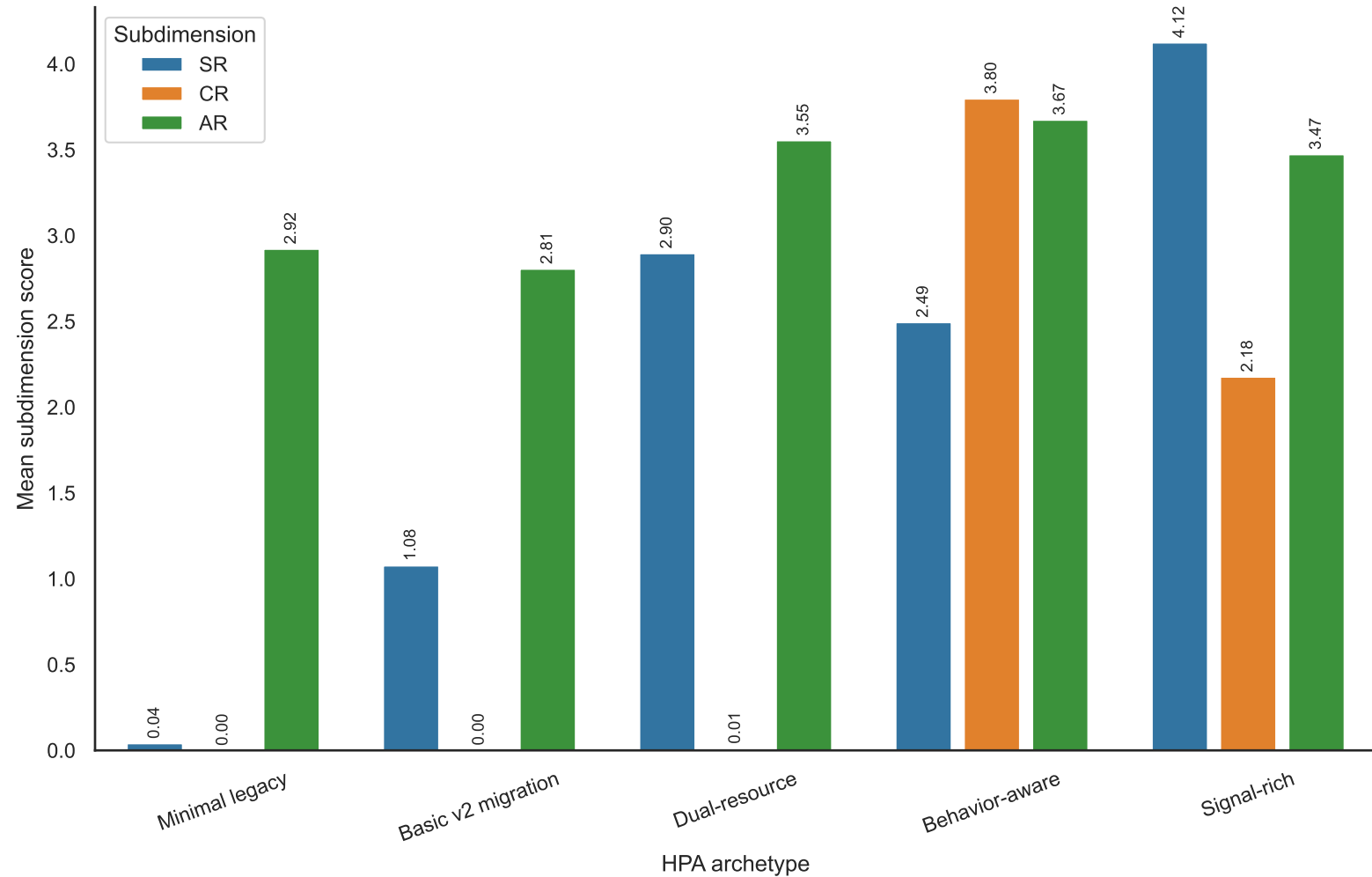
(A) HFRS subdimensions by archetype
