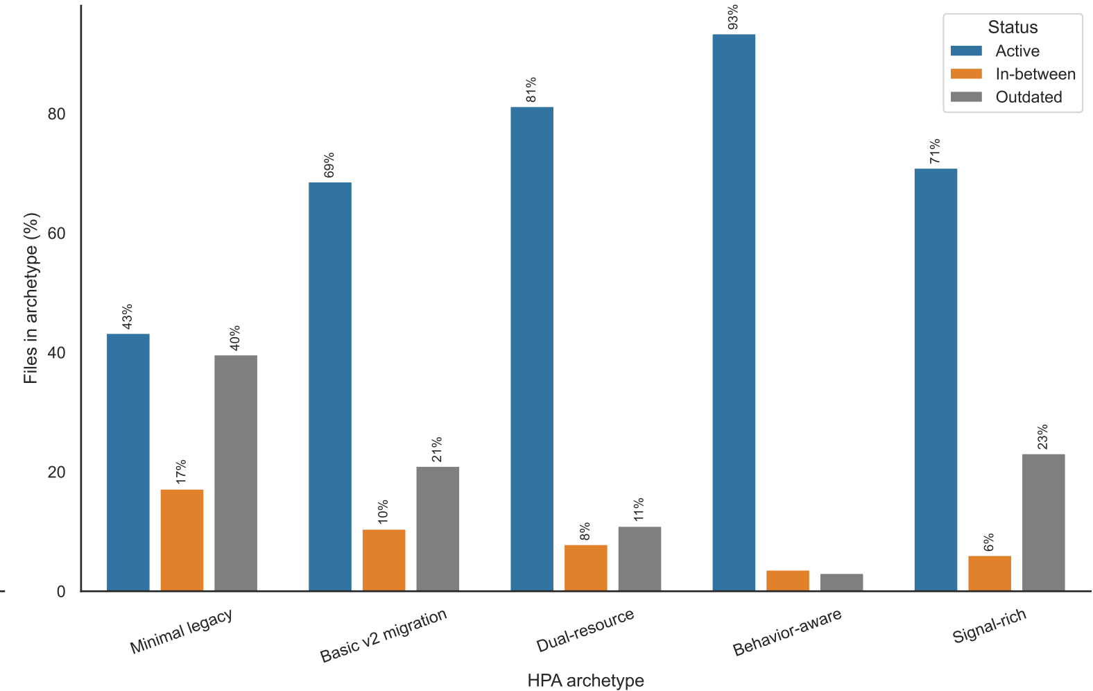
(B) Repository activity status by archetype
