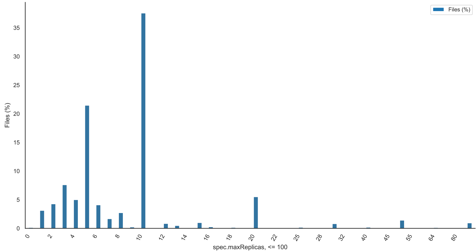
maxReplicas distribution
