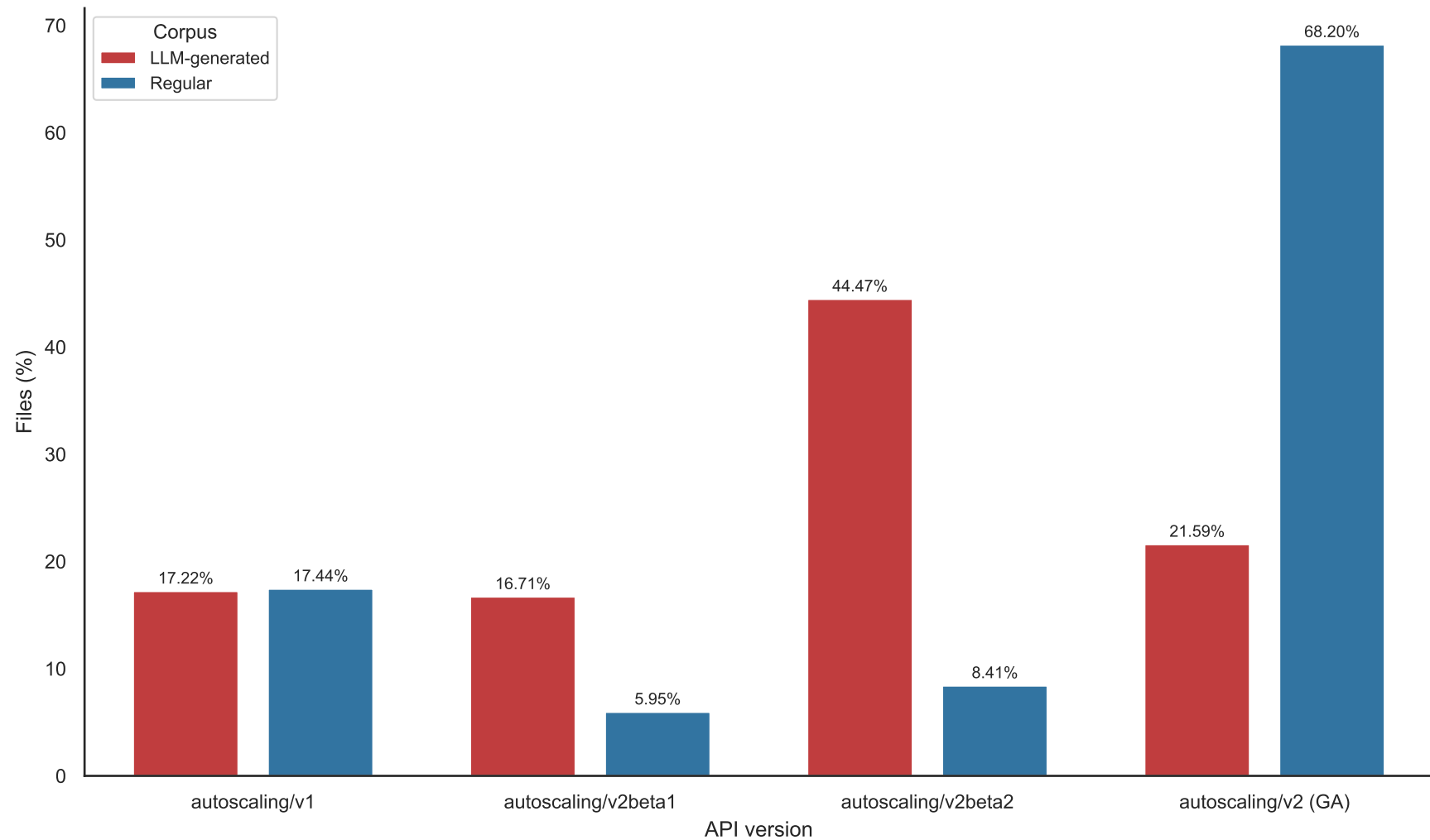
API version distribution, LLM-generated vs. regular files
