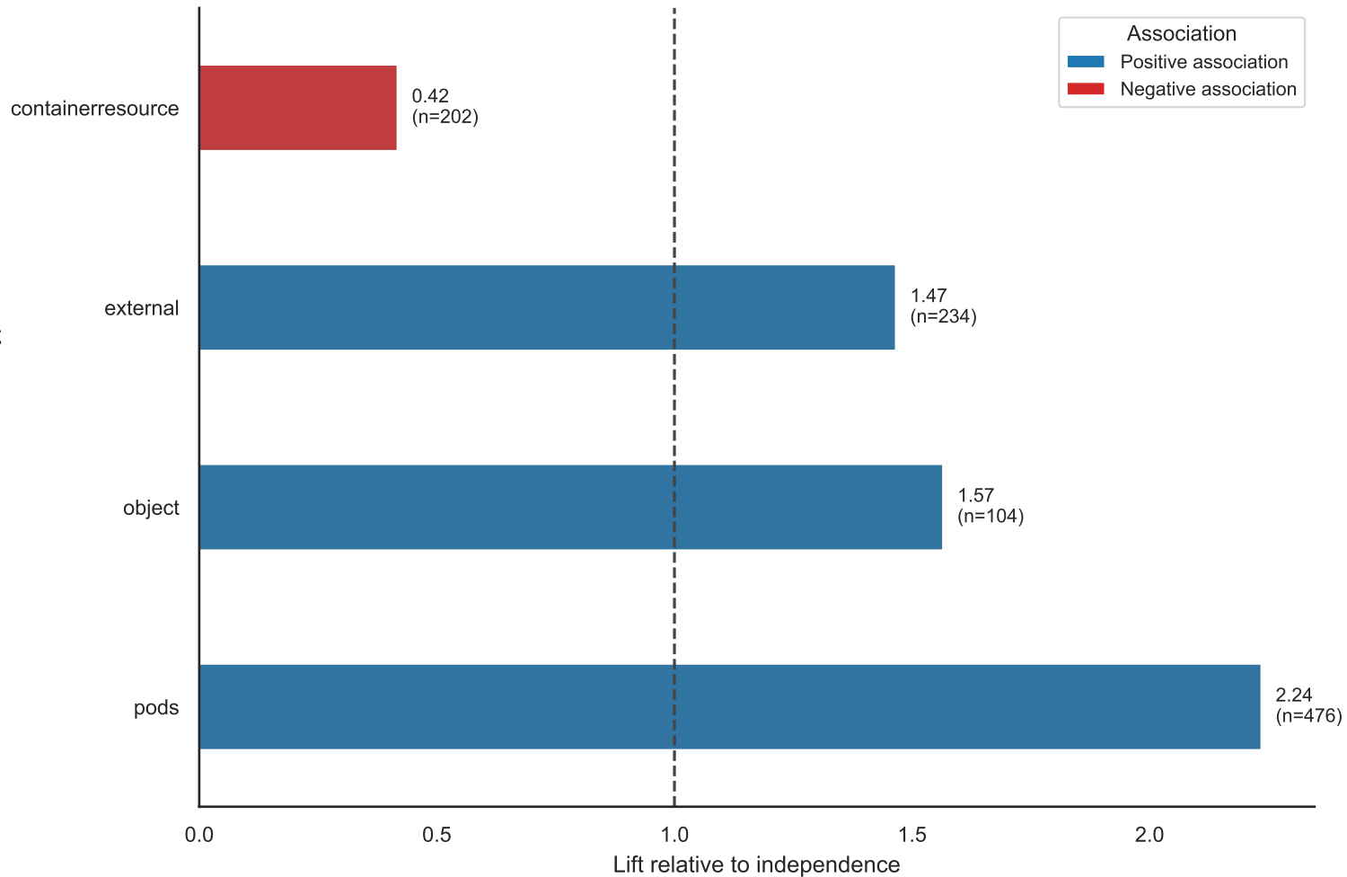
Lift between spec.behavior and each custom metric type
