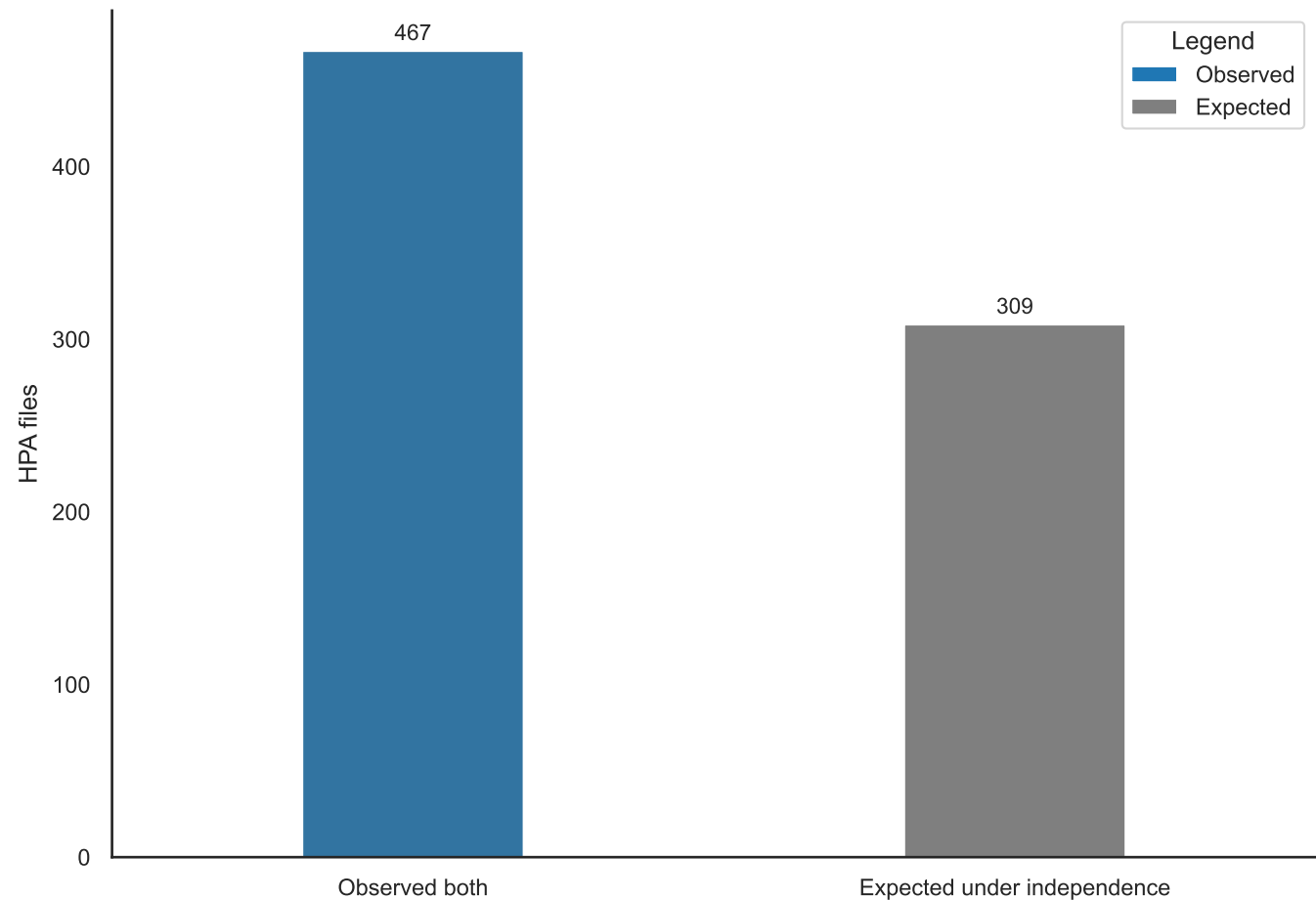
Observed vs expected co-occurrence count
