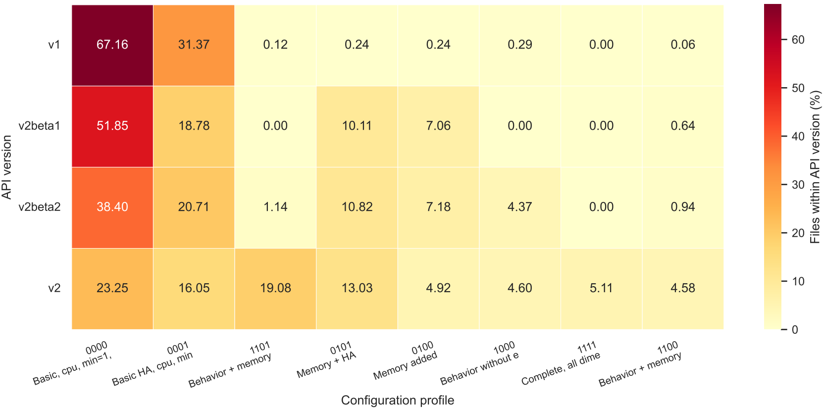
Dominant HPA configuration profiles across API versions
