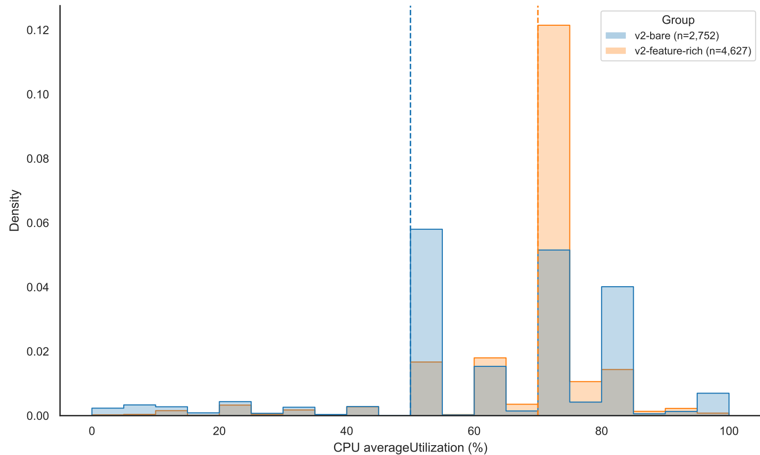
CPU threshold distribution, v2-bare vs. v2-feature-rich
