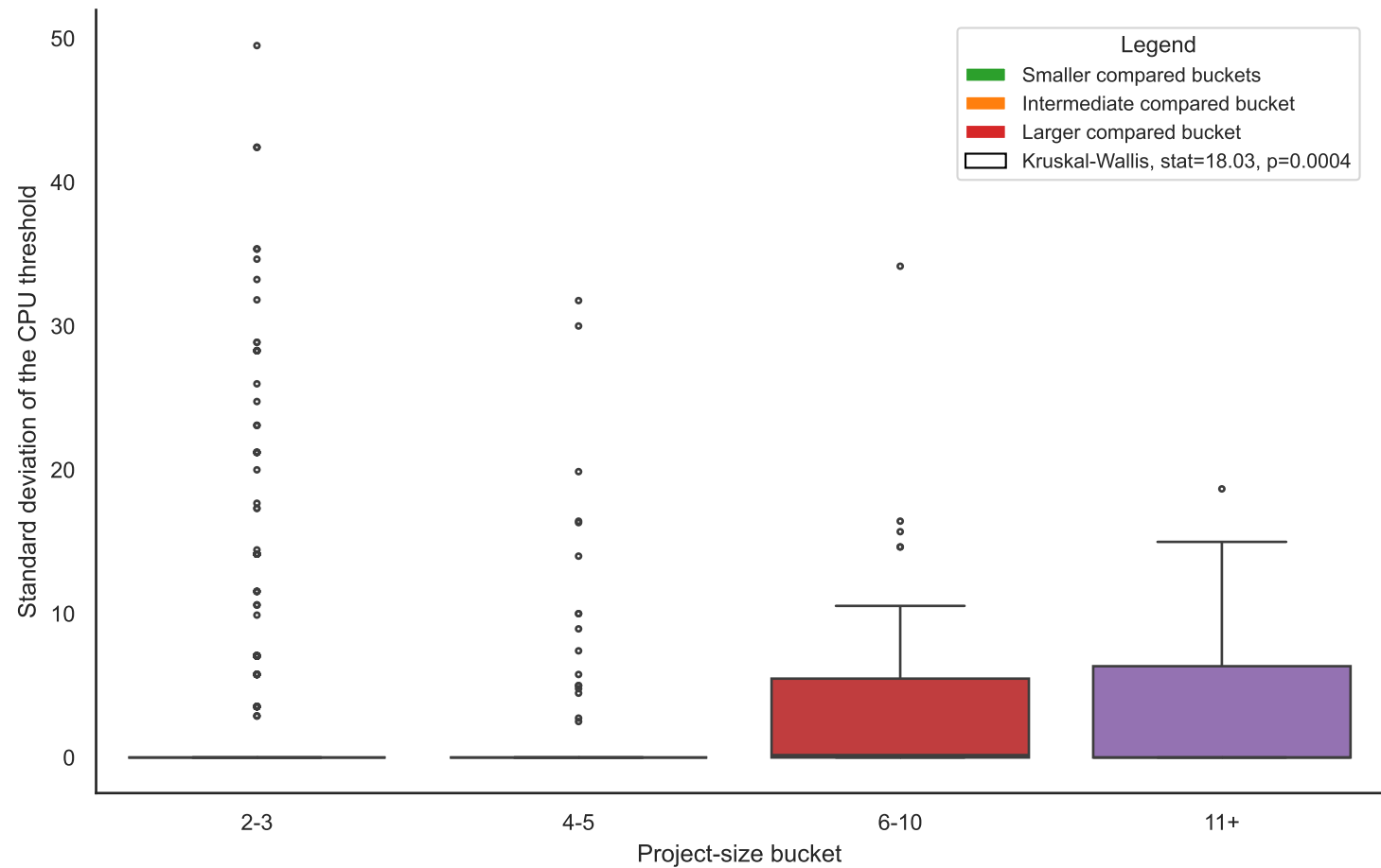
Variation of CPU thresholds across size buckets
