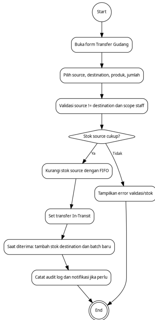
Gambar 4. Activity Diagram Transfer Gudang
