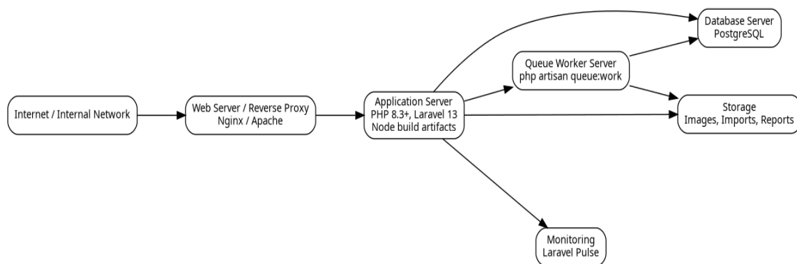
Gambar 8. Hardware Architecture SmartStock Pro
