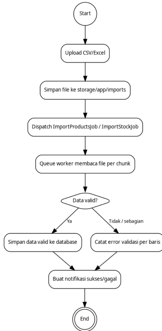
Gambar 5. Activity Diagram Import Data
