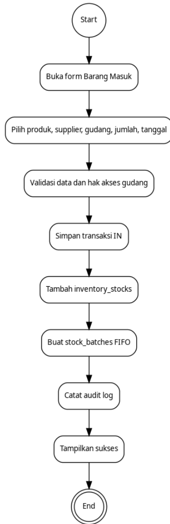
Gambar 2. Activity Diagram Barang Masuk
