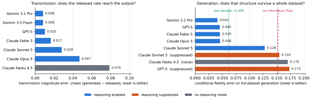
Figure 8: Enterprise-platform generators on one DP release, showing that transmission and generation are different axes. Left: transmission magnitude error, does a released rate reach the output? This panel is the Adult matched-release sweep, not the Diabetes sweep of Appendix H.15.3’s table. Claude Fable 5 reads 0.017 here and 0.009 there. Every platform model is within 0.079 and the best four within 0.017, so on this axis they are near-interchangeable. Right: conditional fidelity on full-dataset generation, against the real-sample reference (0.062) and the no-information floor (0.152). The ordering changes completely. Opus 5 is mid-pack on transmission (0.047) and inside the frontier band on generation (0.046), while Haiku 4.5 is last on both. Bars are coloured by whether reasoning was enabled, suppressed, or unavailable. The three suppressed/absent arms are the ones at or past the no-information floor. The Sonnet 5 reasoning-on bar is the matched arm of Section 7.5 (0.128), not the unmatched run.
