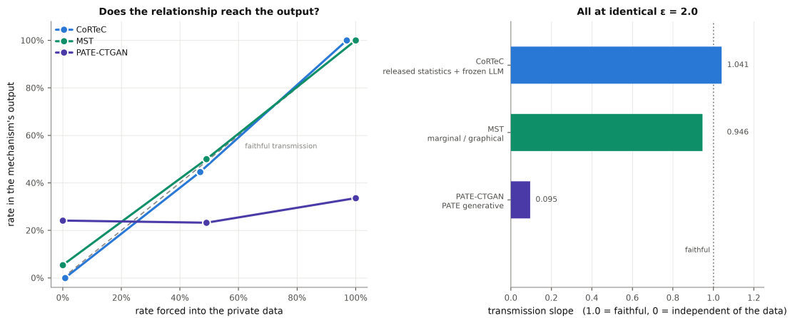
Figure 7: One forced relationship on NHANES (race/ethnicity → diabetes), three mechanisms, identical private data and identical \epsilon = 2.0 . MST and CoRTeC track the diagonal; PATE-CTGAN's output is very nearly flat. The Diabetes 130 rows of the table show the same separation.
