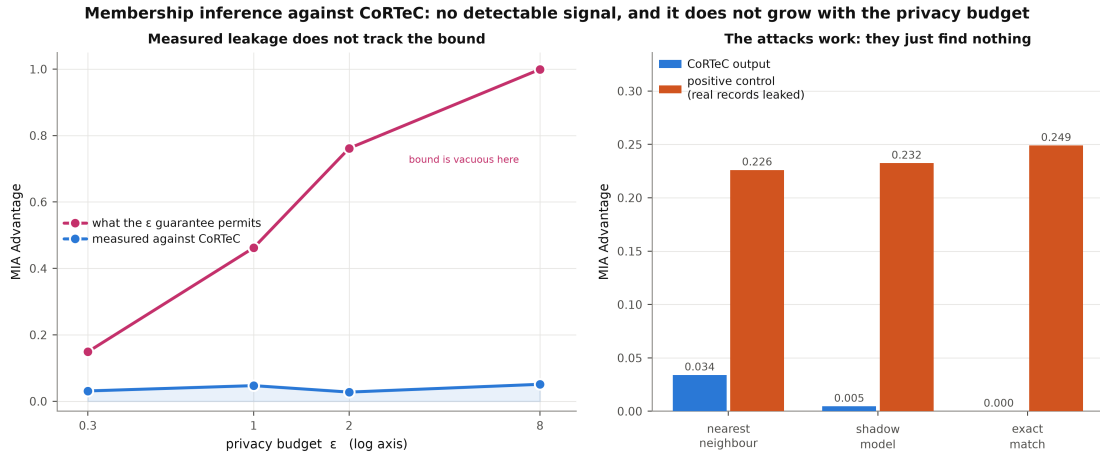
Figure 11: Left: the advantage the \epsilon guarantee permits the advantage measured, across budgets. Right: the attacks against CoRTeC beside the same attacks against a positive control.
