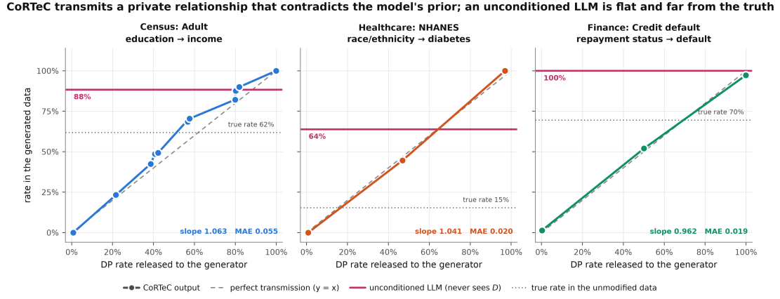
Figure 6: The transmission test. The x-axis is the released rate CoRTeC was given, the y-axis the rate it produced. The dashed diagonal is perfect transmission and the horizontal line is the unconditioned control. The healthcare panel is NHANES.
