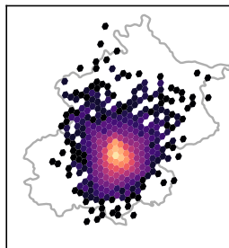
WGAN-GP
