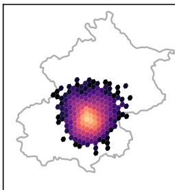
VAE
