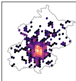
Real
