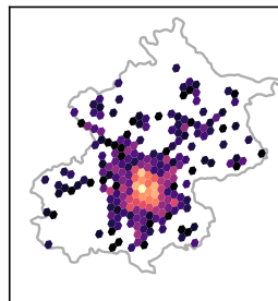
Bootstrap
