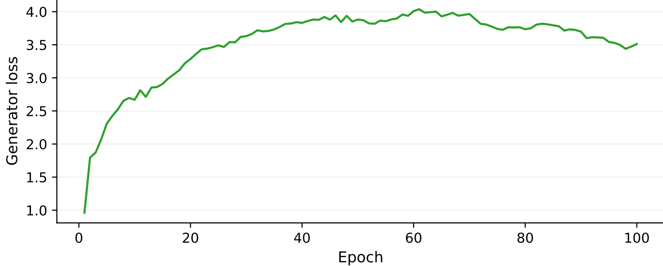
(b) Generator
