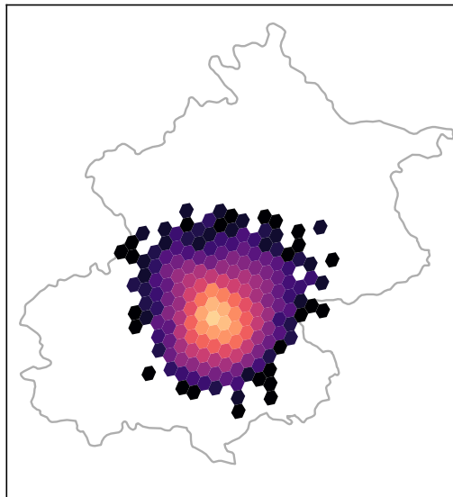
Bootstrap
