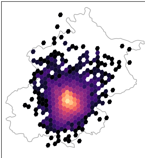
WGAN-GP
