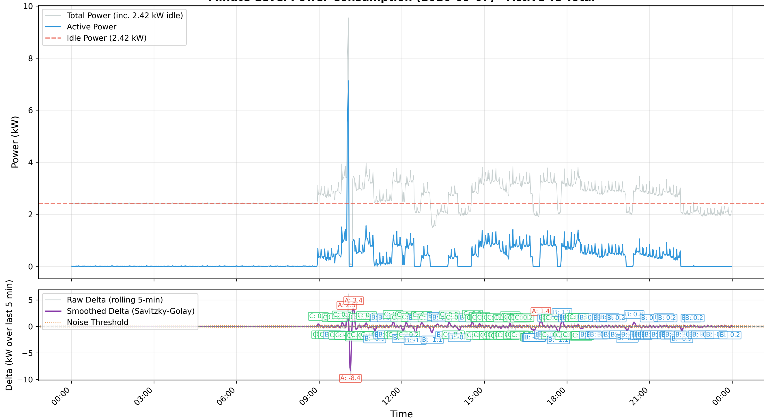
Minute-Level Power Consumption (2026-09-07) - Active vs Total
