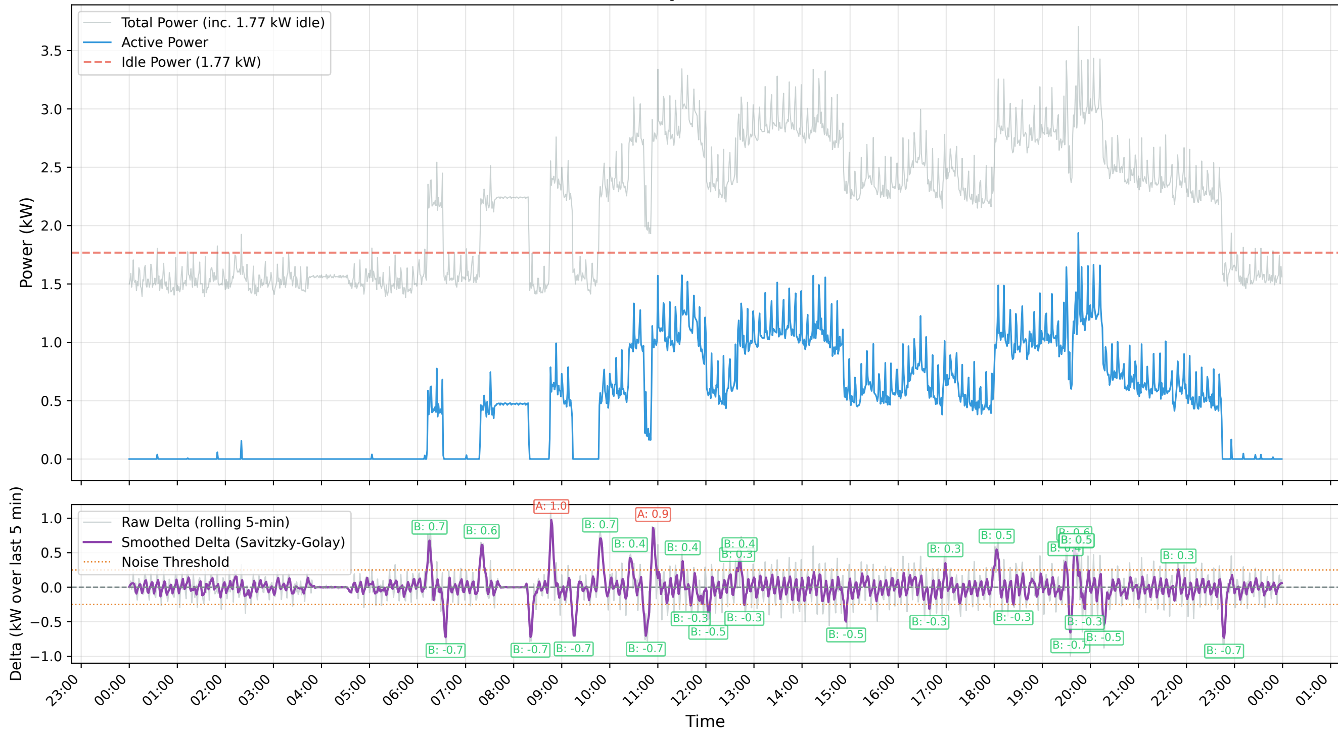
Minute-Level Power Consumption (2026-08-25) - Active vs Total
