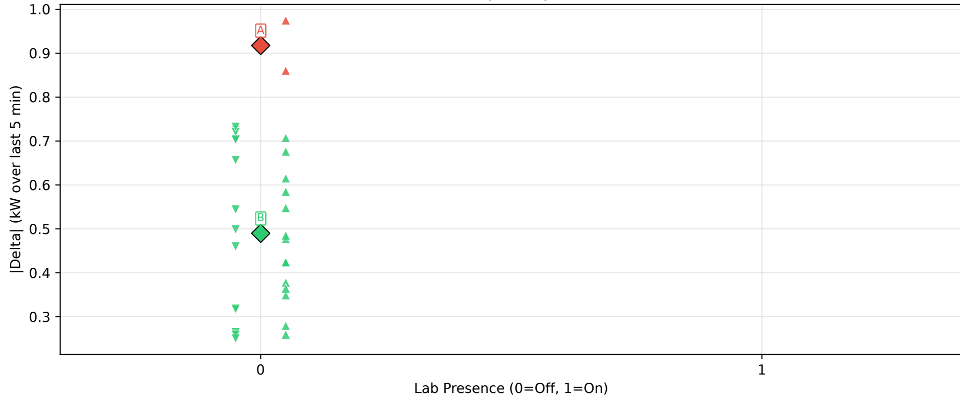
DBSCAN Clusters: Presence vs |\Delta| (eps=0.426, scaled features)
