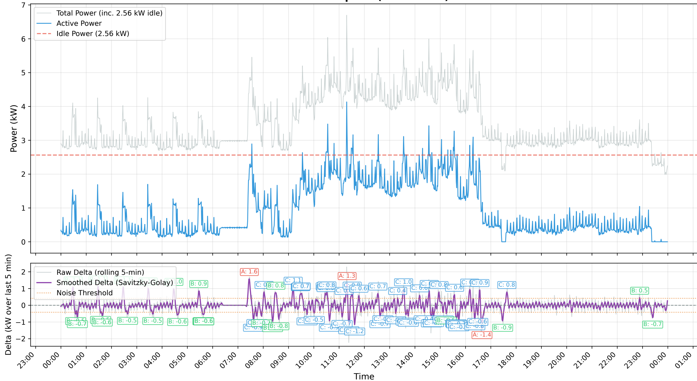
Minute-Level Power Consumption (2026-08-10) - Active vs Total
