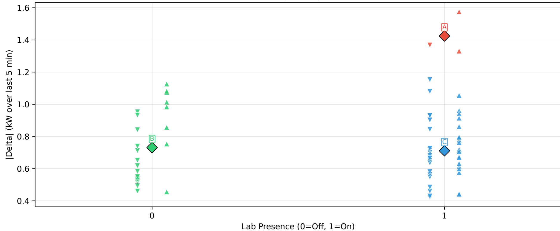
DBSCAN Clusters: Presence vs |Delta| (eps=0.574, scaled features)
