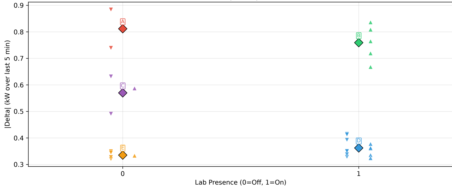
DBSCAN Clusters: Presence vs |Delta| (eps=0.553, scaled features)
