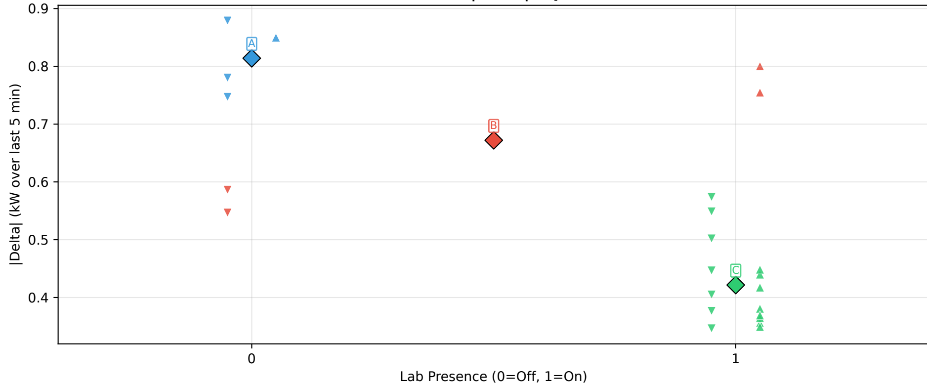
DBSCAN Clusters: Presence vs |Delta| (eps=0.641, scaled features)
