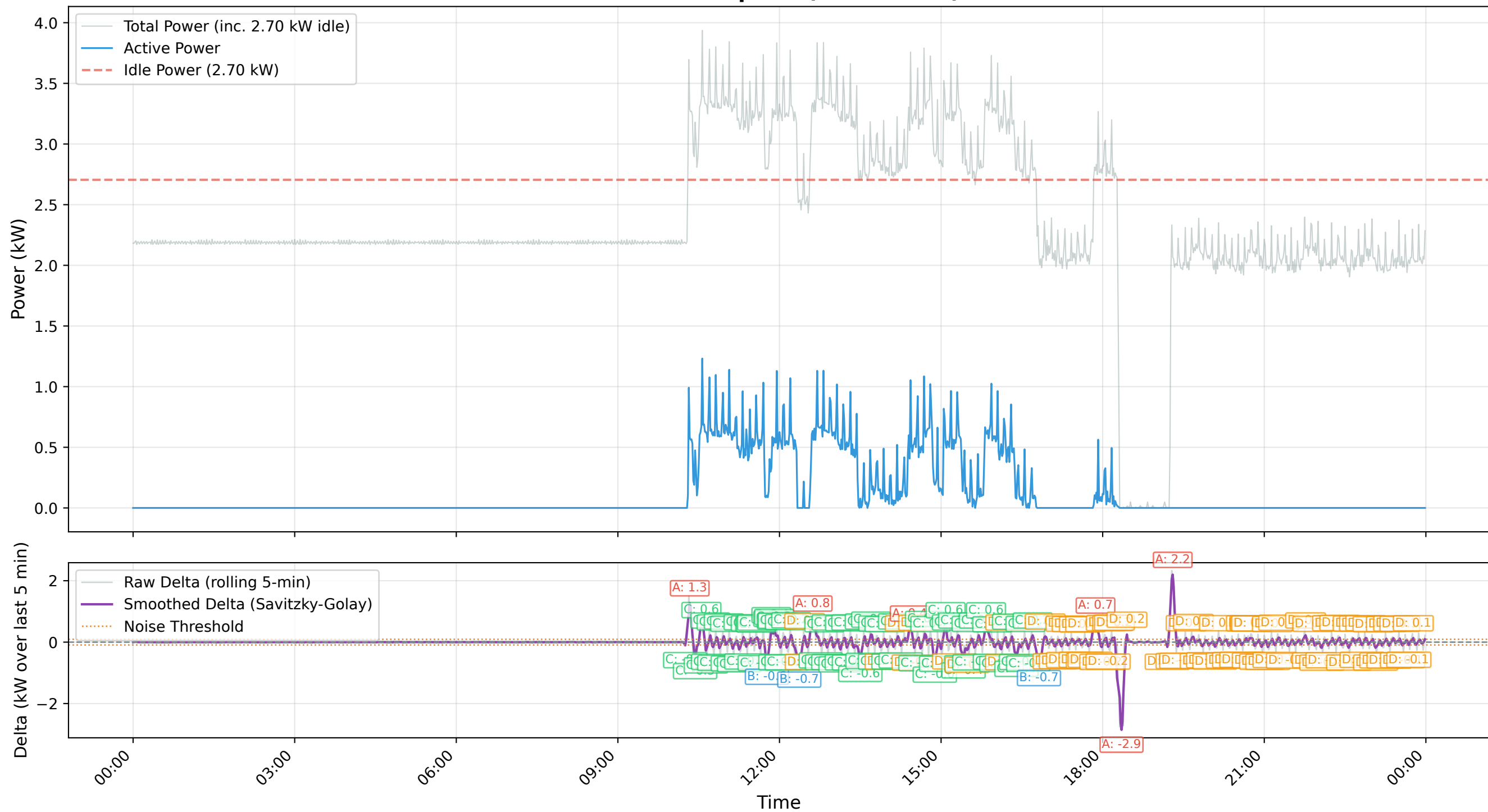
Minute-Level Power Consumption (2026-09-15) - Active vs Total
