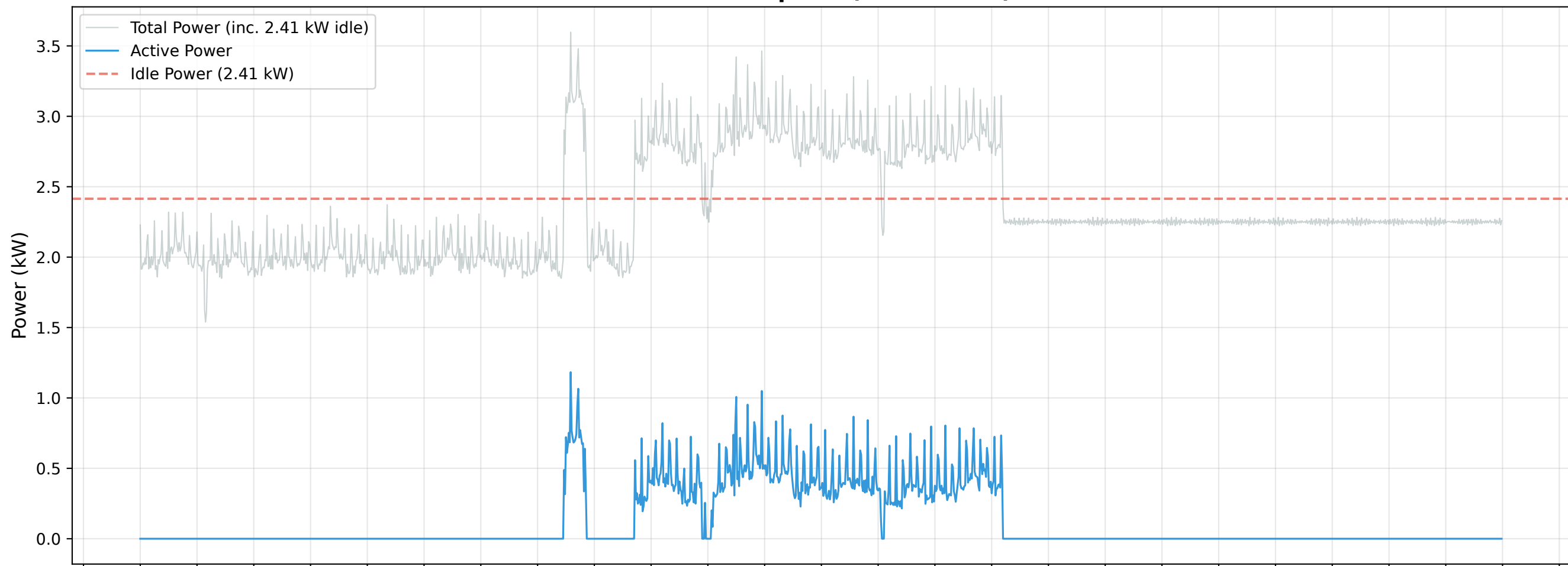
Minute-Level Power Consumption (2026-07-30) - Active vs Total
