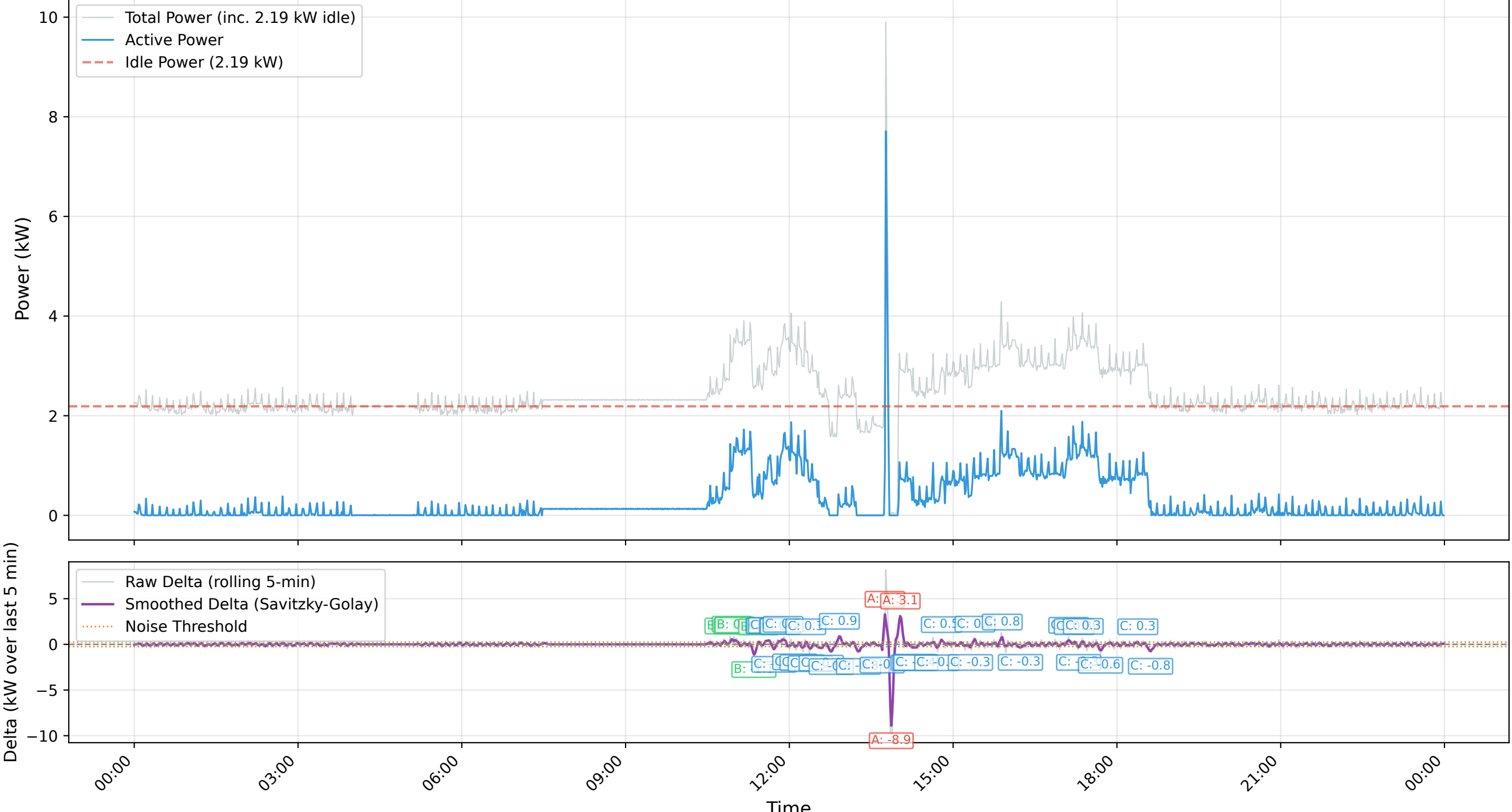
Minute-Level Power Consumption (2026-10-07) - Active vs Total
