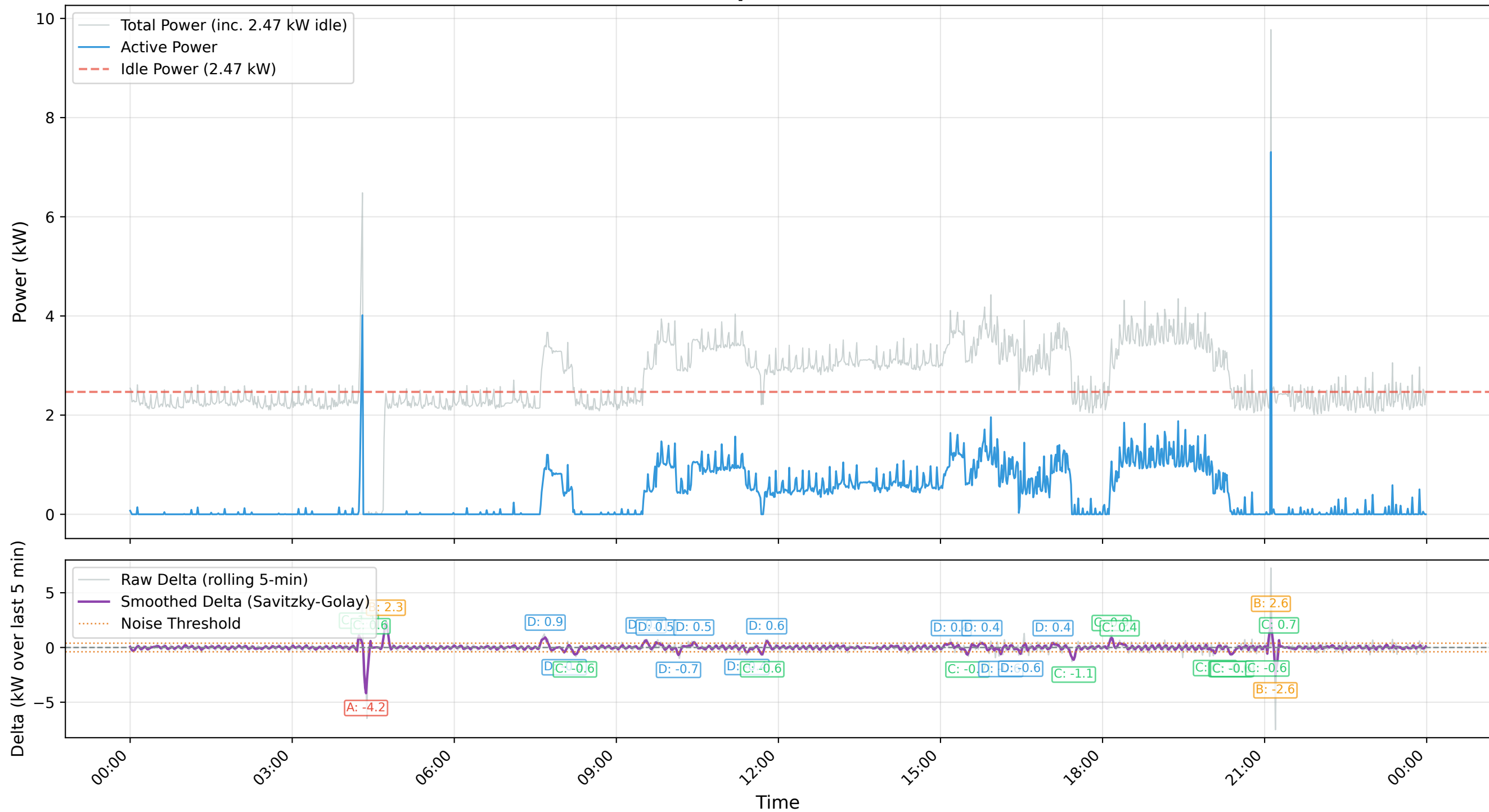
Minute-Level Power Consumption (2026-09-28) - Active vs Total
