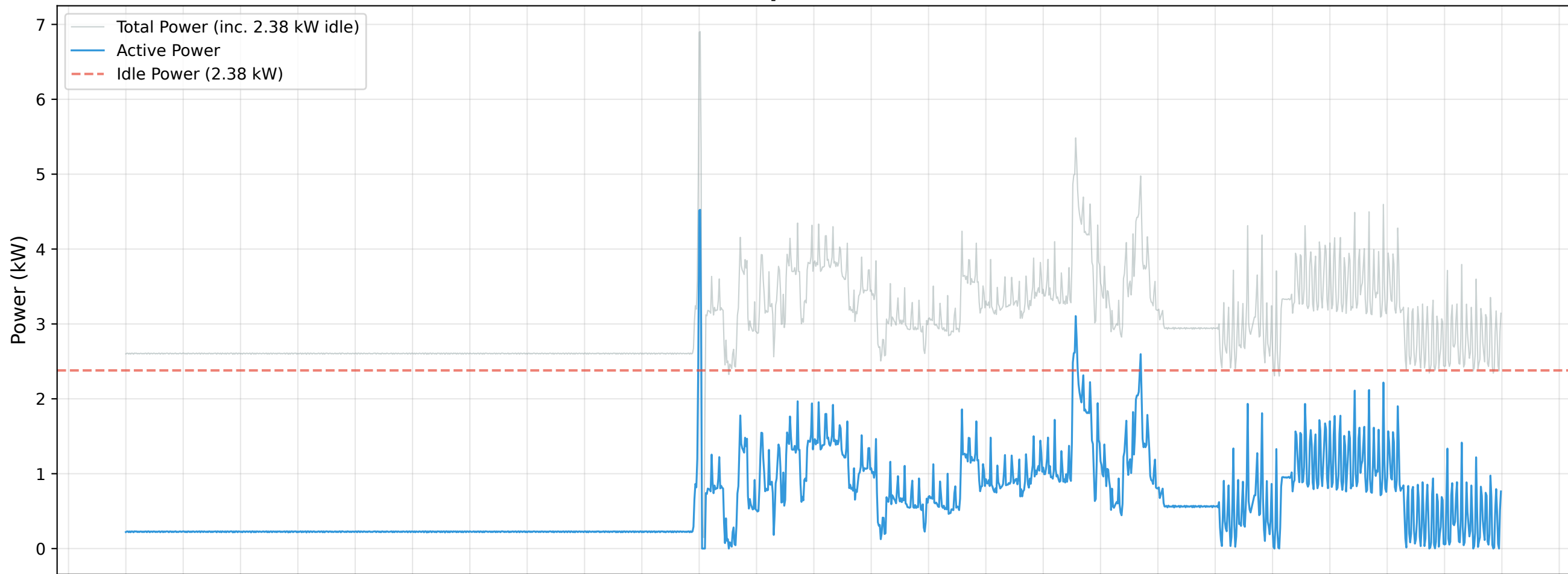
Minute-Level Power Consumption (2026-07-24) - Active vs Total
