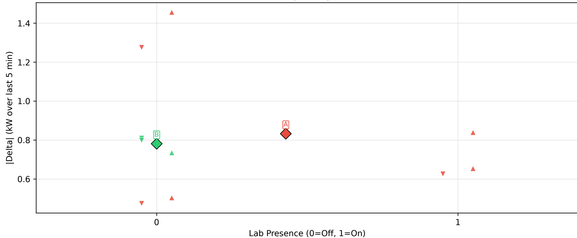
DBSCAN Clusters: Presence vs |\Delta| (eps=0.443, scaled features)
