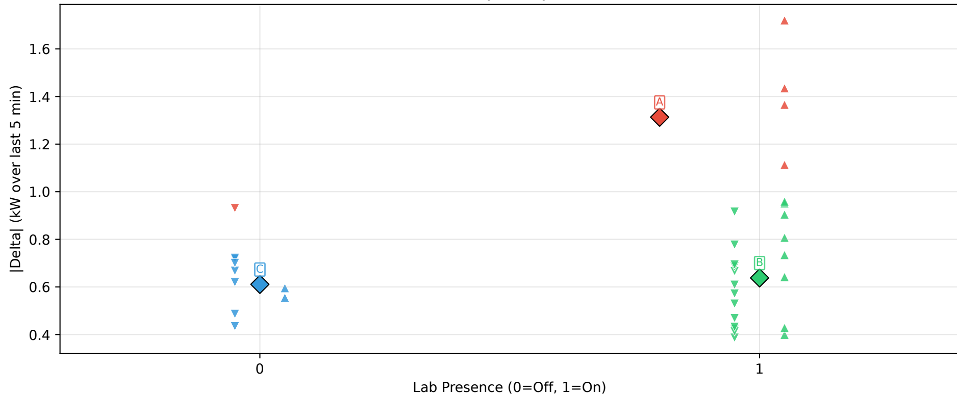
DBSCAN Clusters: Presence vs |Delta| (eps=0.413, scaled features)
