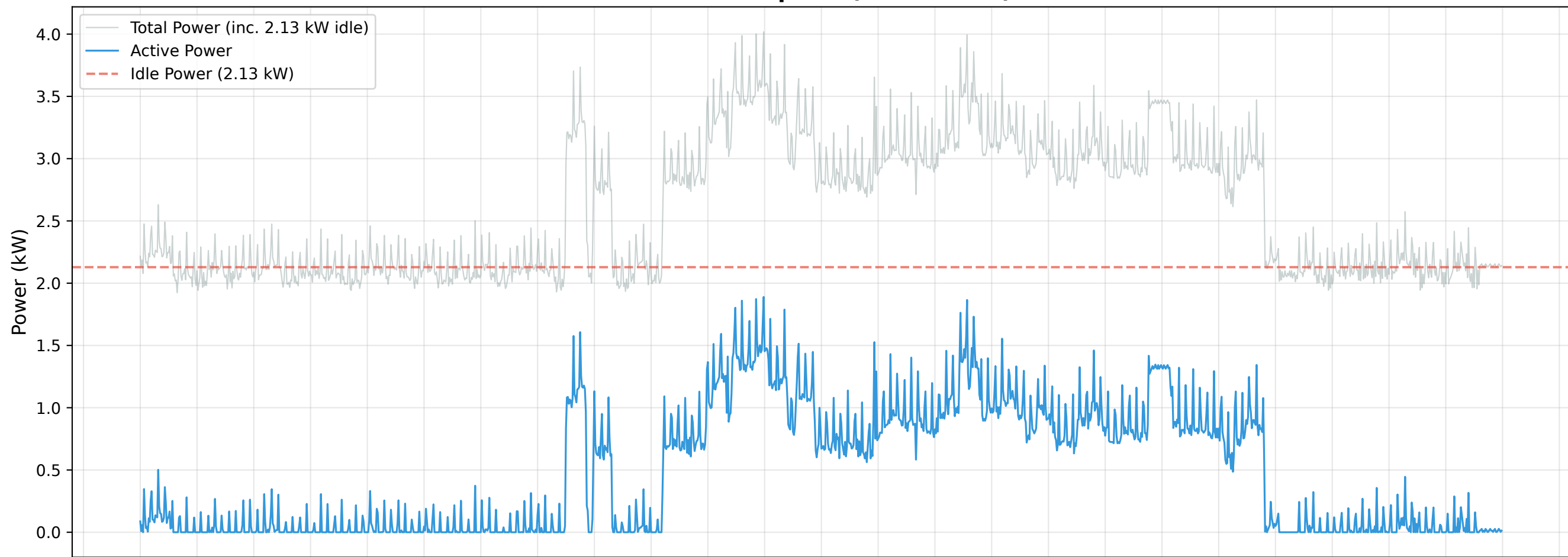
Minute-Level Power Consumption (2026-08-06) - Active vs Total
