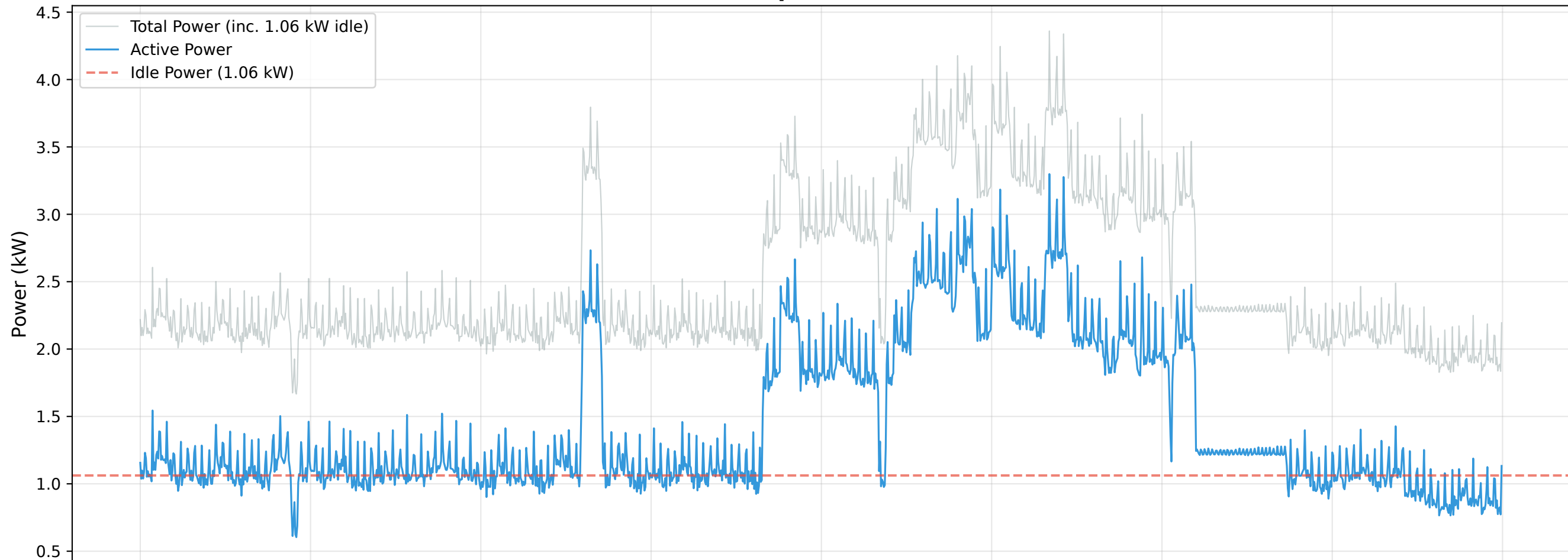
Minute-Level Power Consumption (2026-09-23) - Active vs Total
