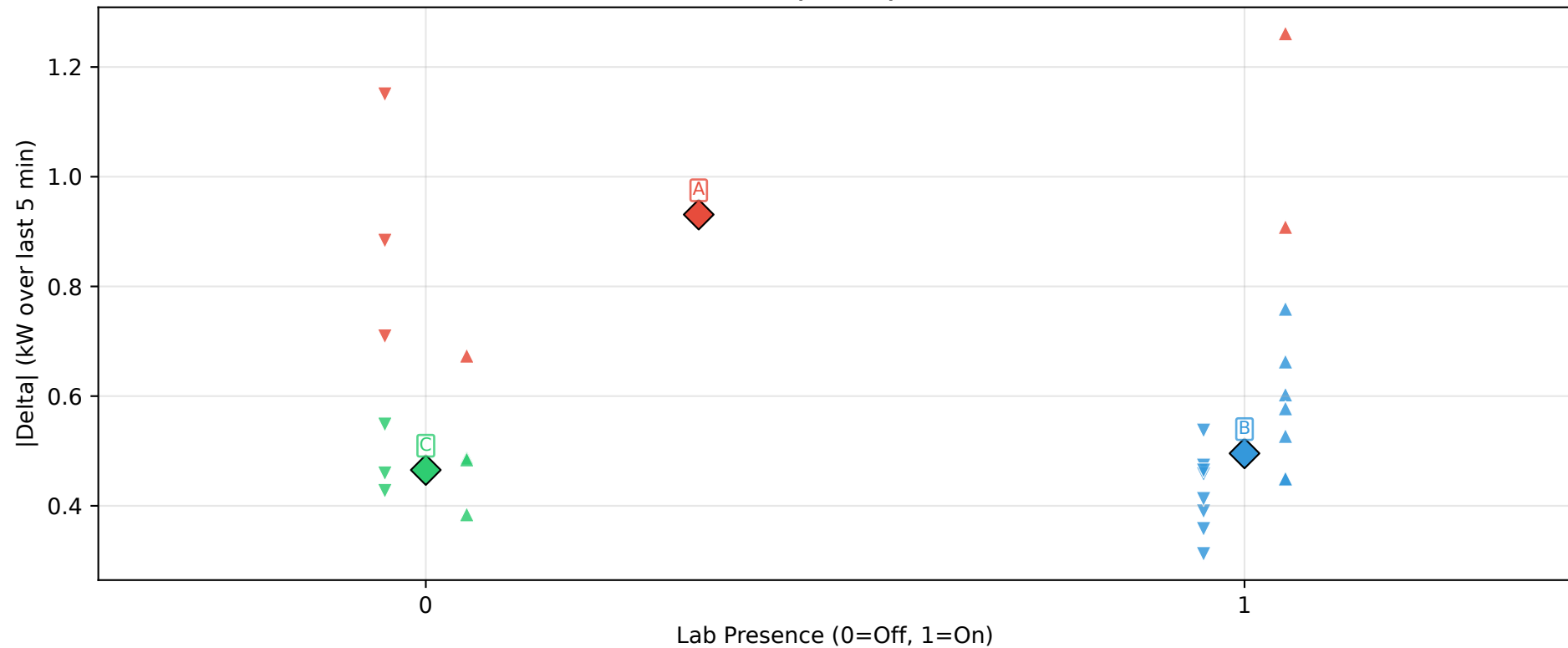
DBSCAN Clusters: Presence vs |\Delta| (eps=0.435, scaled features)
