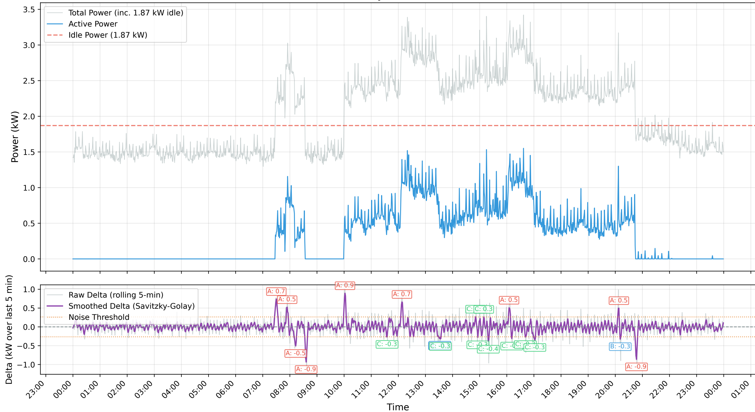
Minute-Level Power Consumption (2026-08-24) - Active vs Total
