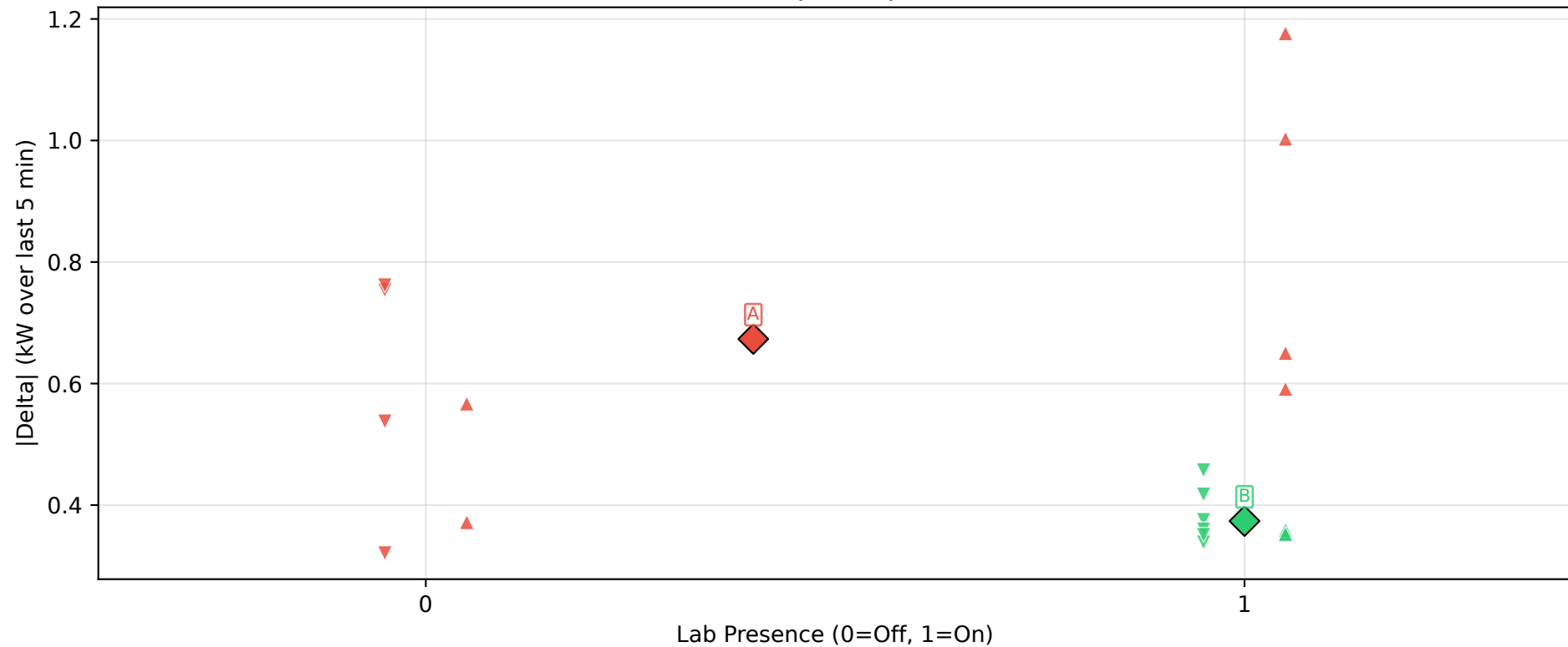
DBSCAN Clusters: Presence vs |Delta| (eps=0.431, scaled features)
