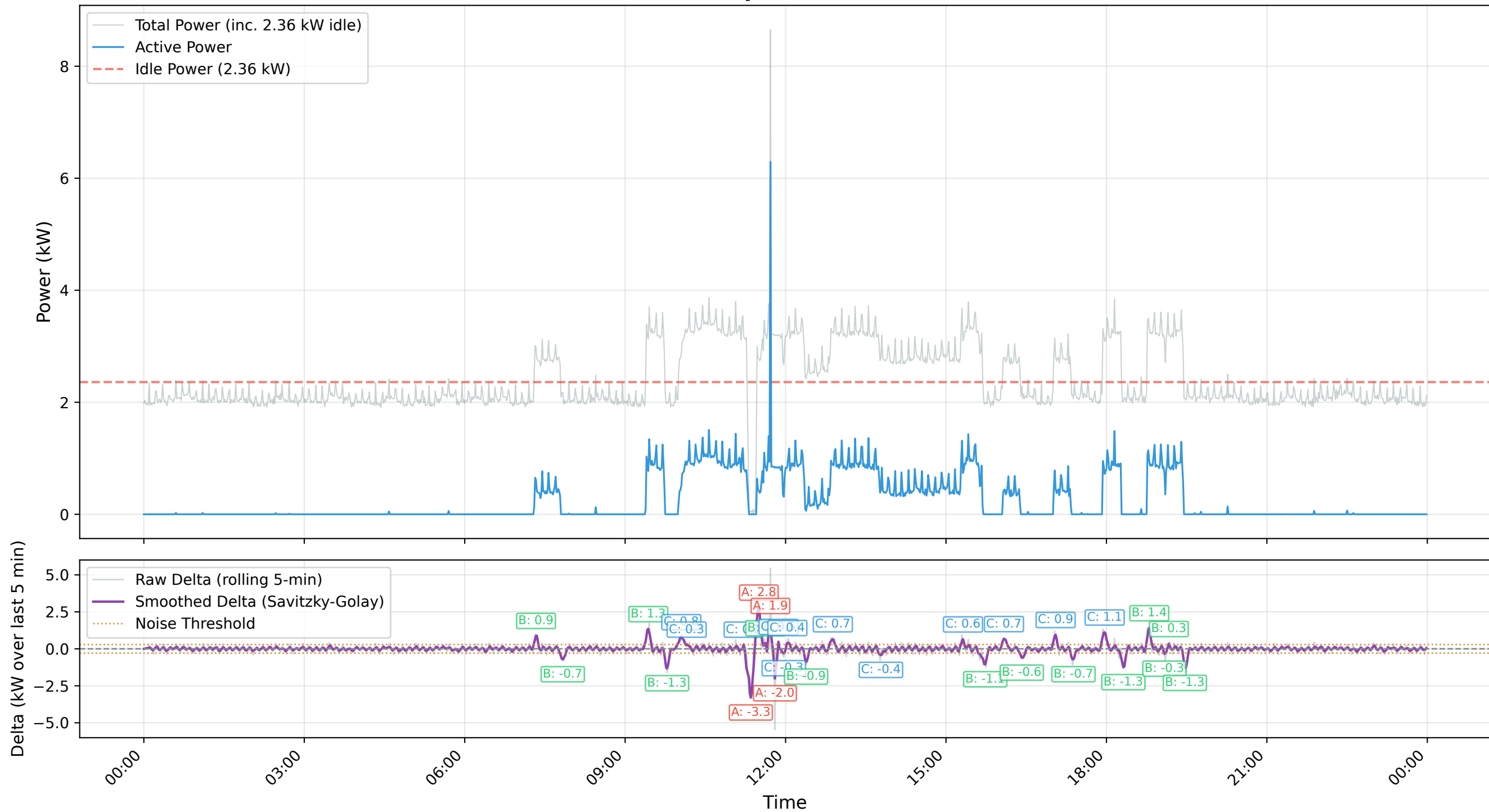
Minute-Level Power Consumption (2026-09-08) - Active vs Total
