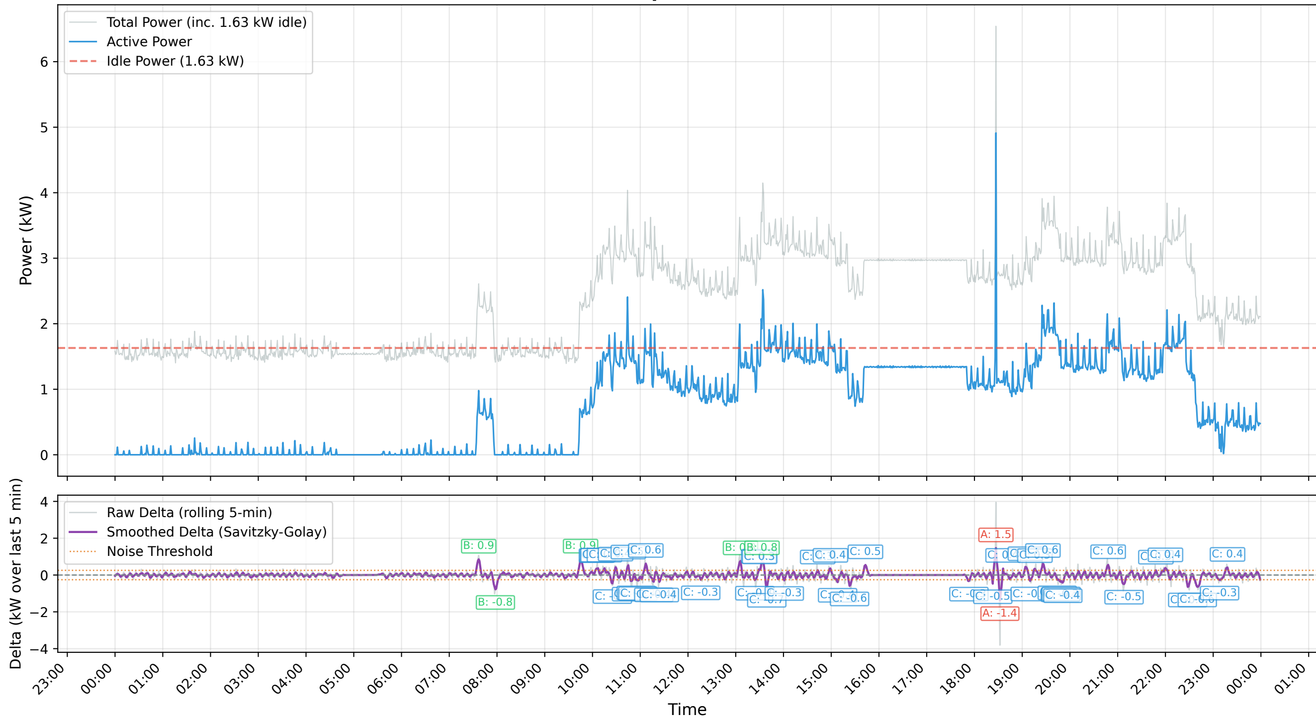
Minute-Level Power Consumption (2026-08-26) - Active vs Total
