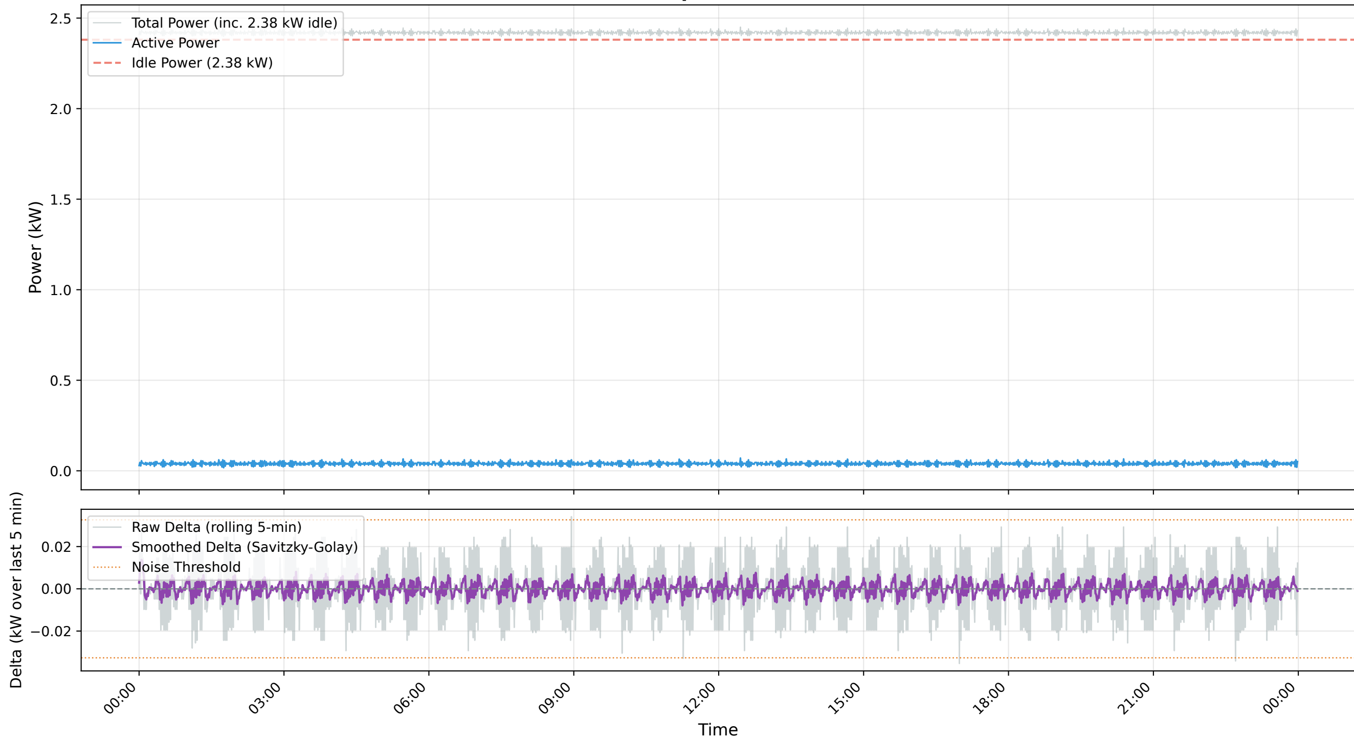
Minute-Level Power Consumption (2026-09-04) - Active vs Total
