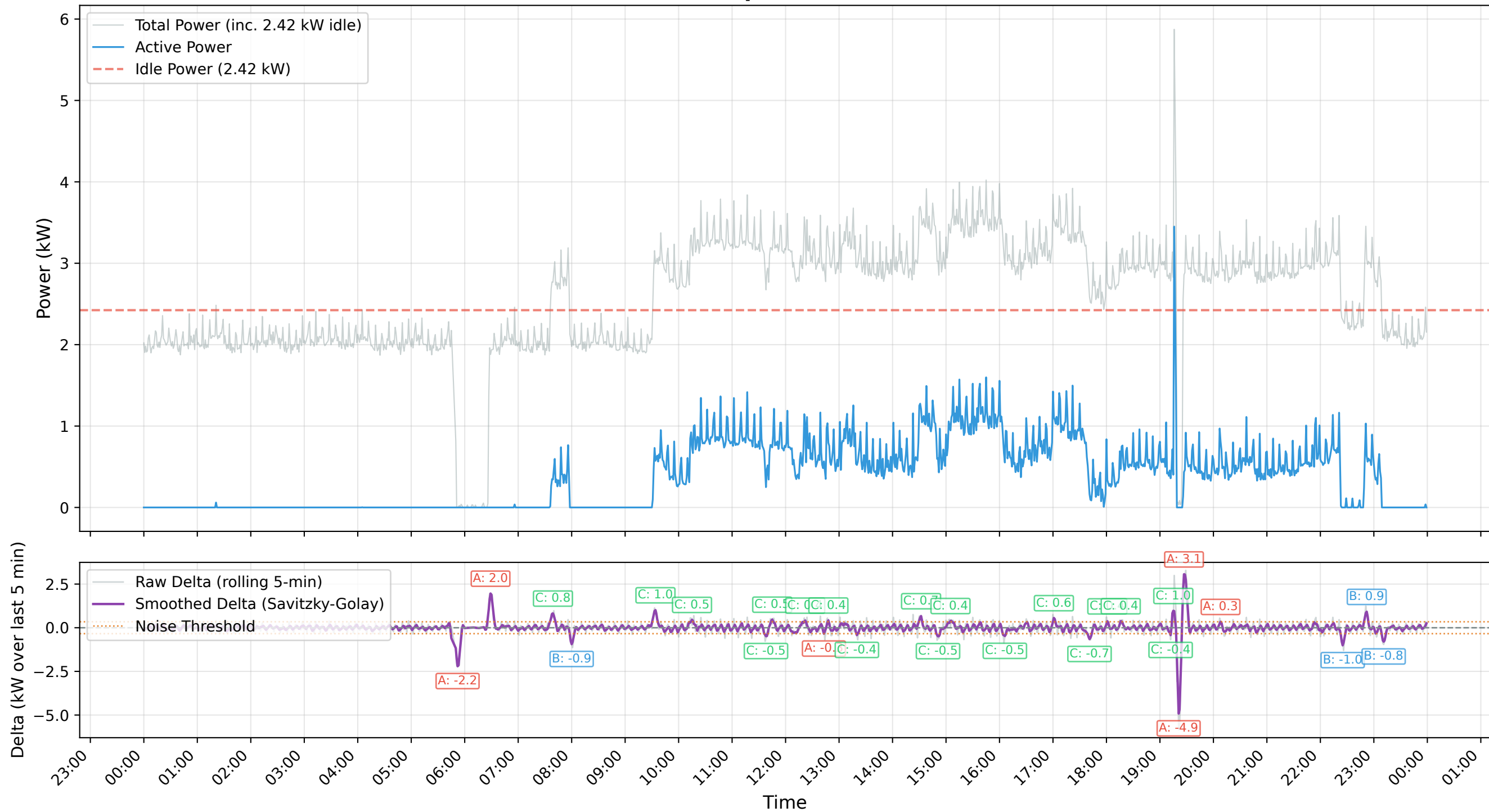
Minute-Level Power Consumption (2026-08-13) - Active vs Total
