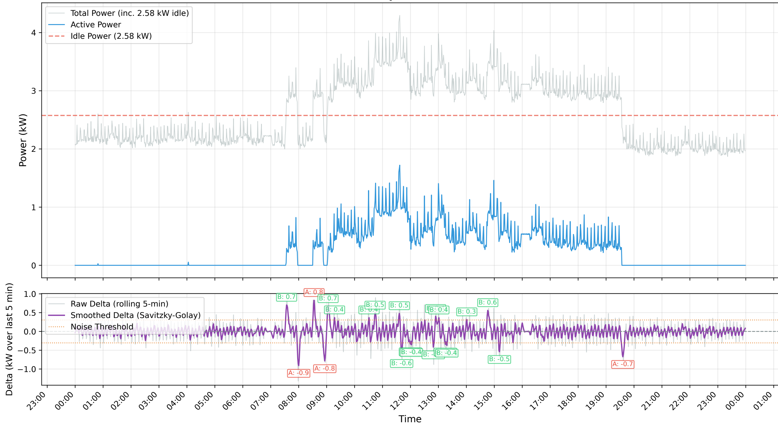
Minute-Level Power Consumption (2026-07-28) - Active vs Total
