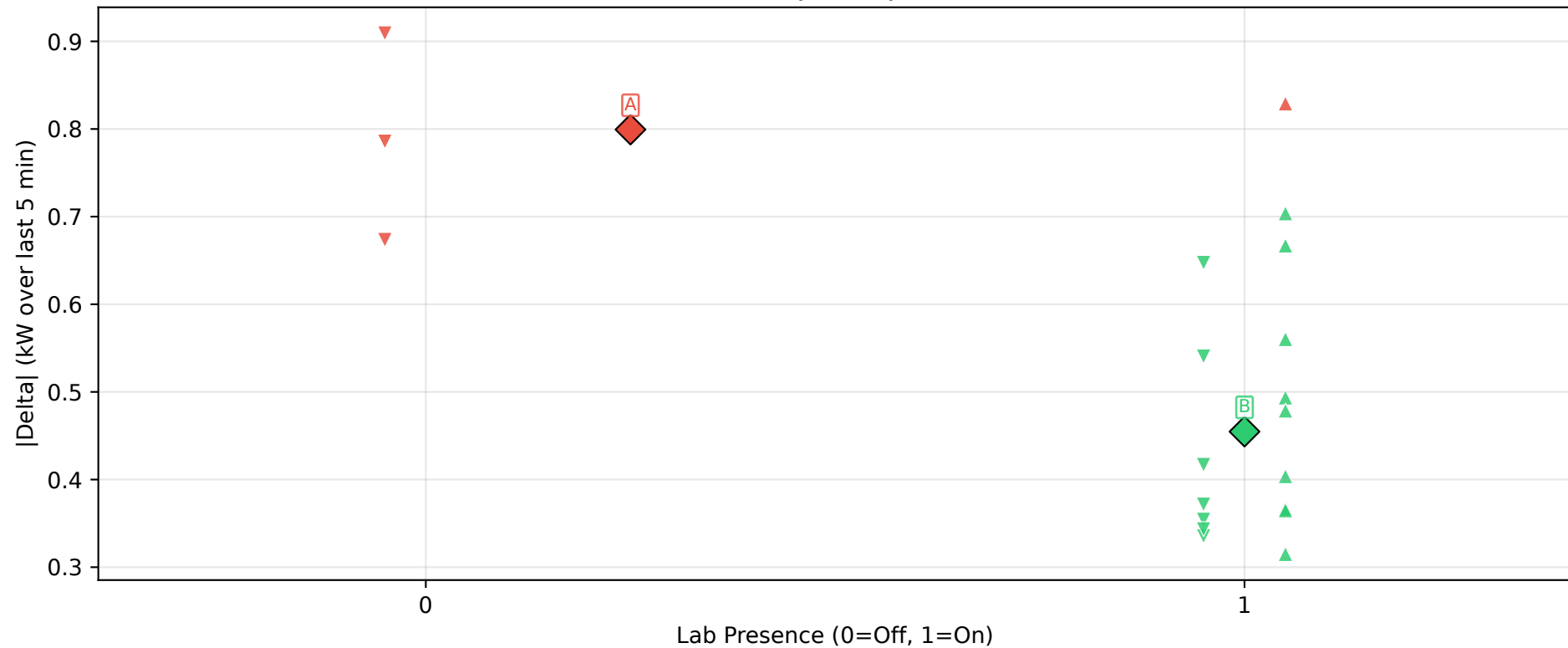
DBSCAN Clusters: Presence vs |Delta| (eps=0.563, scaled features)
