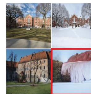
Style transfer
