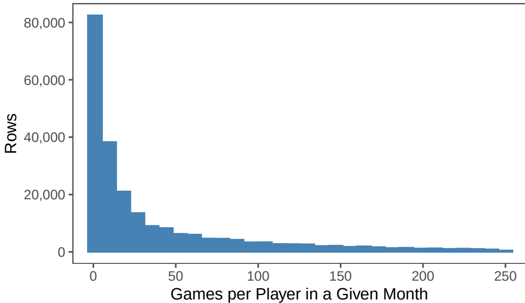
Player-Month Reliability Varies Widely
