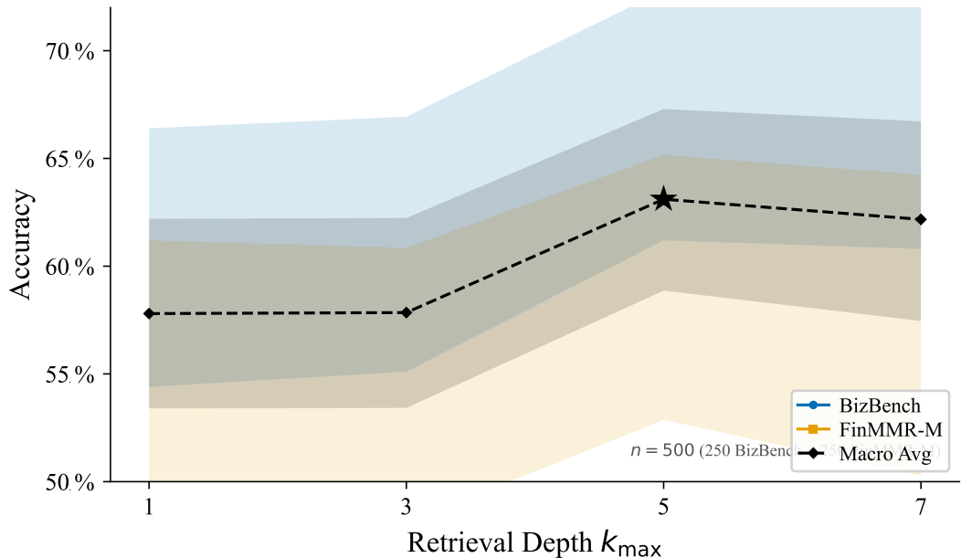
Accuracy vs. Retrieval Depth k_{\max}
