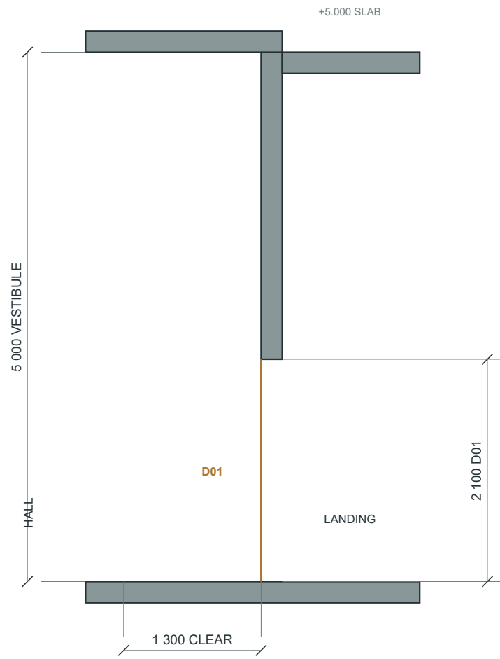
D01 / ENTRY SECTION
