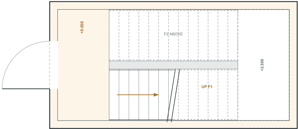
03 / LEVEL +0.000
