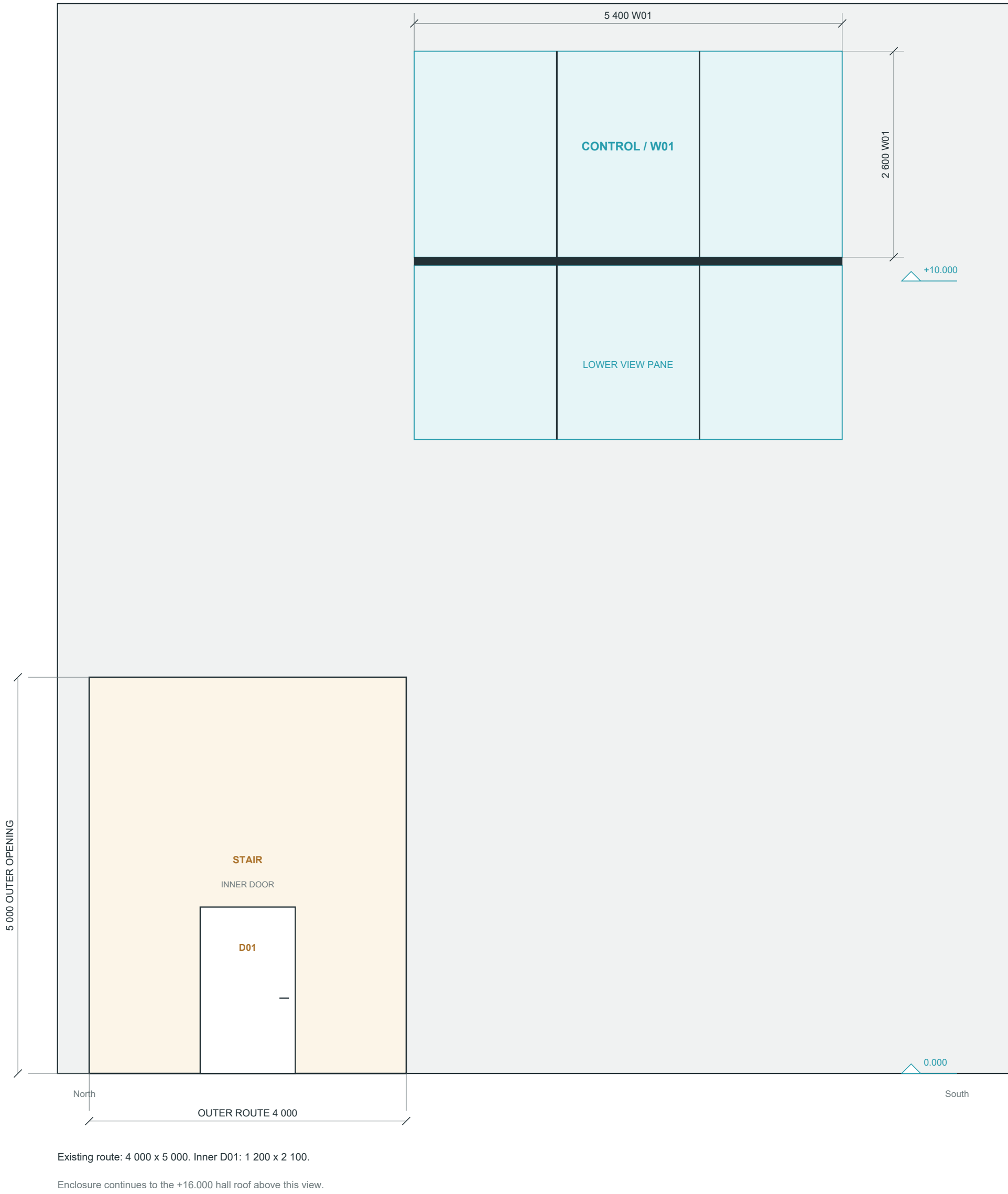
E01 / EAST WALL - VIEWED FROM HALL
